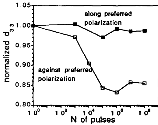
Figure 5. Normalized piezoelectric coefficient at E = 230 \text{ kV/cm} as a function of number of voltage pulses ( 300 \text{ KV/cm} ) applied along and against the direction of preferred polarization.
