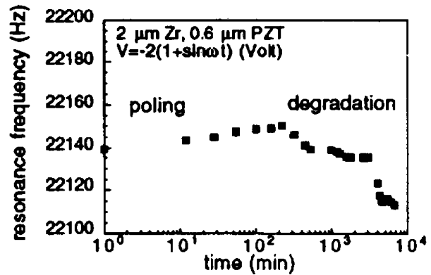
Figure 6. Resonance frequency of a Zr membrane covered by 0.6 \mu\text{m} PZT film showing degradation under the conditions imitating the work of a piezoelectric ultrasonic motor.
