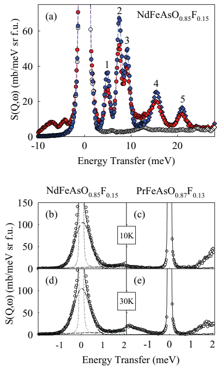
FIG. 4. (Color) (a) Inelastic neutron-scattering spectra of NdFeAsO _{0.85} F _{0.15} measured on Merlin with incident energies of 15 meV (circles) and 35 meV (diamonds) at an average Q of 1 \text{ \AA}^{-1} and temperatures of 7 K (blue symbols) and 50 K (red symbols). Open symbols are nonmagnetic scattering from LaFeAsO _{0.85} F _{0.15} . (b)–(e) The inelastic neutron-scattering data measured on the IN6 with an incident energy of 3.1 meV and an average elastic Q of 0.65 \text{ \AA}^{-1} for NdFeAsO _{0.85} F _{0.15} [(b) and (d)] and PrFeAsO _{0.87} F _{0.13} [(c) and (e)] at 10 K [(b) and (c)] and 30 K [(d) and (e)]. The dotted line in (b) and (d) and the solid line in (c) and (e) are the elastic nuclear scattering. In (b) and (d), the dashed line is the quasielastic Gaussian line shape fit, and the solid line is the sum of elastic nuclear, magnetic, and small linear background contributions.
