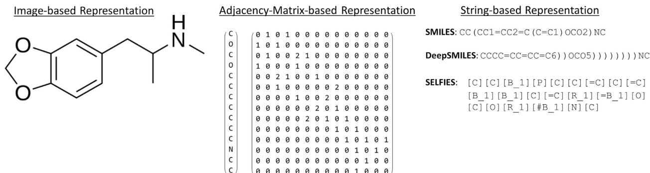
Figure 13. Graphs can be represented in numerous ways, for example using images, adjacency matrices, or strings. All of them are graph representations. By relating string-based representations to programming languages, we show that they are in general the most expressive representations. For SELFIES, B1 and R1 are abbreviations for Branch1 and Ring1, respectively.
