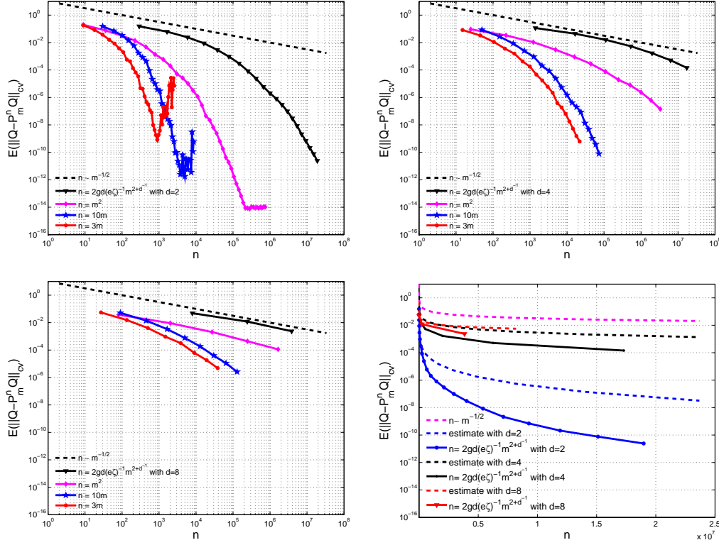
FIGURE 3. Error \mathbb{E}(\|Q - \tilde{P}_m^n Q\|_{cv}) , testing different relations between the number of samples n and the dimension of the polynomial space m . Top-left: d = 2 . Top-right: d = 4 . Bottom-left: d = 8 . Bottom-right: comparison between the numerical results and the theoretical bound (116), with d = 2 , d = 4 and d = 8 .
