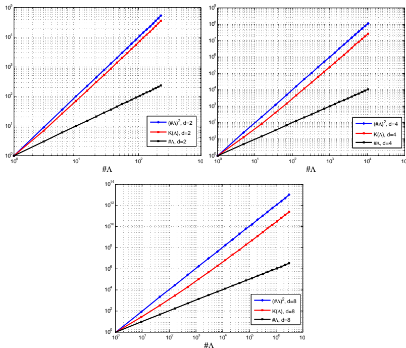
FIGURE 1. Comparison between \#(\Lambda) , K_L(\Lambda) and (\#(\Lambda))^2 in the case where \Lambda = S_{k,d} (see (66)). Left: d = 2 . Center: d = 4 . Right: d = 8 .
