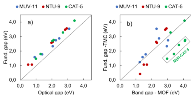
Figure 5. (a) Correlation between the fundamental gap and optical gap of the M-TMCs computed with PBE0. (b) Correlation between the band gap of the solid MOFs and the representative TMCs computed with PBE0 at the PBE-D3BJ optimized geometries.
