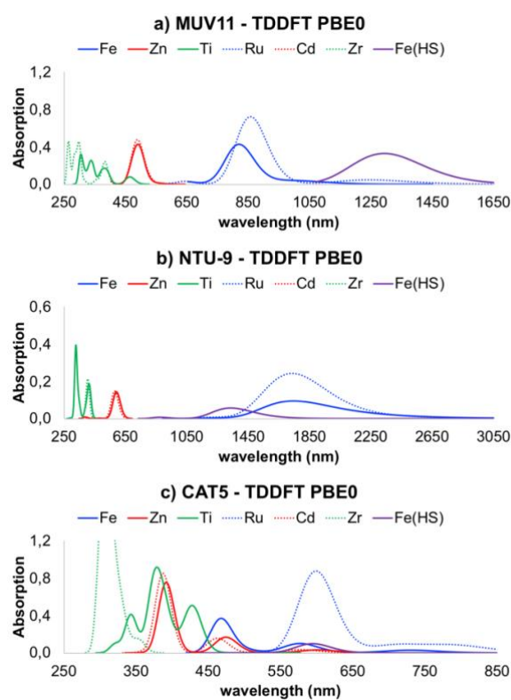
Figure 4. LR-TDDFT absorption spectra computed with PBE0 functional for (a) MUV-11, (b) NTU-9 and (c) CAT-5 TMCs. The absorption intensity of Fe(HS) is shown x3 to make it visible. Thin/dashed lines are used for 1 st /2 nd row TMCs.
