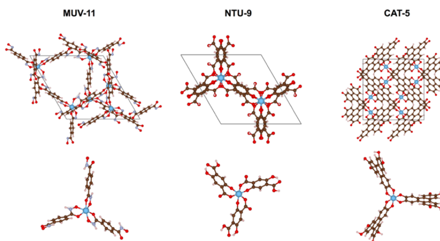
Figure 1. Crystal structure (top) and cluster structure (bottom) of the 3 studied Ti(IV)-MOFs: MUV-11 built from benzene-1,4-dihydroxamate ligand, NTU-9 built from 2,5-dihydroxyterephthalate ligand and CAT-5 built from triphenylene-2,3,6,7,10,11-hexakis(olate) ligand.
