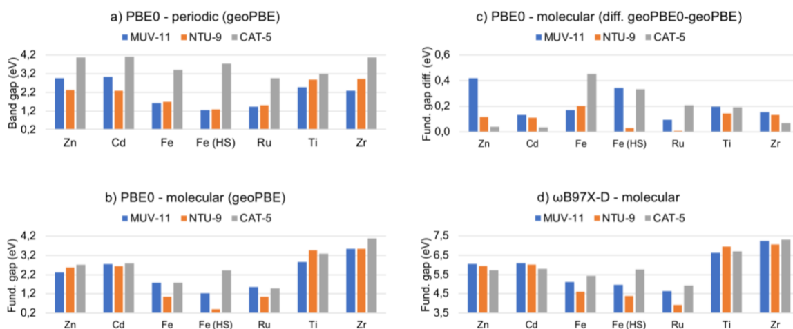
Figure 3. (a) PBE0 band gap given in eV computed for the MOF periodic crystals at their optimized PBE-D3BJ geometry and (b) fundamental gap for the molecular compounds. (c) Fundamental gap difference between the PBE0 values at the PBE0-D3BJ and PBE-D3BJ geometries of the TMCs. (d) Fundamental gap values computed for the TMCs at the \omega B97X-D level. Raw data in Table S4 and S5.
