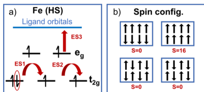
Figure 8. Schematic representation of a) the HS electronic configuration of Fe(II)-TMCs indicating the three lowest excited states (ES) computed with LR-TDDFT and b) the different spin configurations that can arise in Fe(II)-MOFs.
