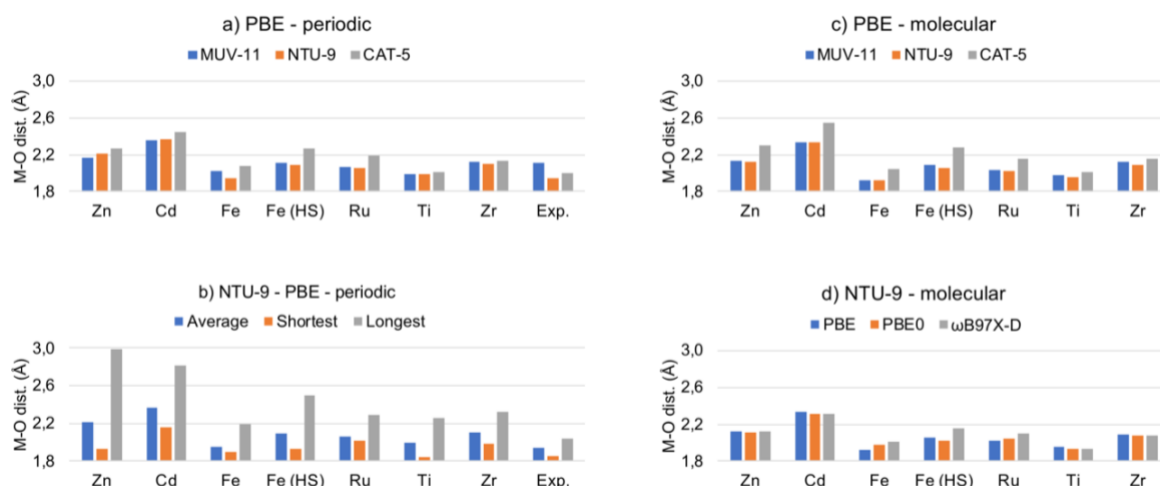
Figure 2. (a) Average metal-oxygen (M-O) distances in Å of the PBE-D3BJ optimized MOF crystals. (b) Average, shortest and longest M-O distances of the PBE-D3BJ optimized NTU-9 MOF. (c) Average M-O distances of the TMCs optimized at the PBE-D3BJ level. (d) Average M-O distances of NTU-9 TMCs optimized with PBE-D3BJ, PBE0-D3BJ and \omega B97X-D. Raw data is given in Table S2 and S3.
