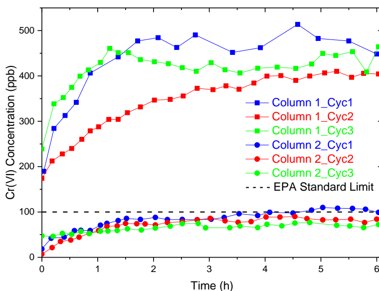
Fig 5. (a) The process flow diagram of the gas-sparged adsorption/photoreduction system (inset) column regeneration with HCl solution under irradiation (b) Cr(VI) concentration at the outlet of adsorption-photoreduction system (square) column 1 (circle) column 2 for three consecutive cycles.
