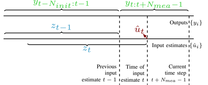
Fig. 1: Diagram of input estimation at time t . Input estimate \hat{u}_t can be estimated after y_{t+N_{mea}-1} is measured at time t+N_{mea}-1 . Differently, output prediction \bar{y}_{t+1} is computed immediately by (2), if given u_{t+1} .
