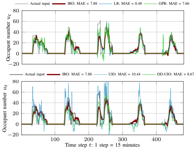
Fig. 4: Comparison of occupant number estimation. Top: MH-IRO, LR and GPR. Bottom: MH-IRO, UIO and DD-UIO. Mean absolute error (MAE) is computed for the data during office hours.
