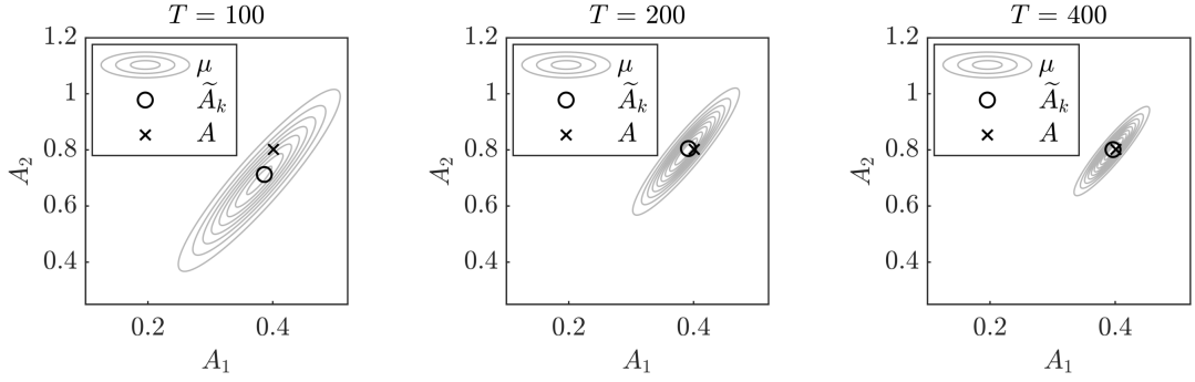
Figure 6: Results for Section 5.3. Posterior distributions over the parameter A = (A_1, A_2)^\top for the bistable potential obtained with the filtered data approach. The figures refer to final time T = 100, 200, 400 from left to right, respectively. The MLE \tilde{A}_k(X^\varepsilon, t) is represented with a circle, while the true value A of the drift coefficient of the homogenized equation is represented with a cross.
