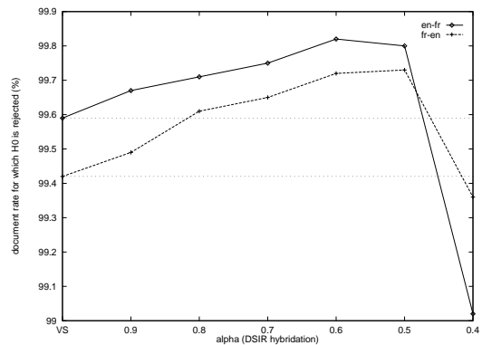
Figure 2: Impact of the hybrid DSIR model on the validation of the relevance of a vector-based similarity in a multi-lingual framework
