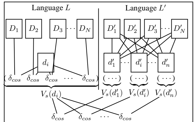
Figure 1: Validation method
