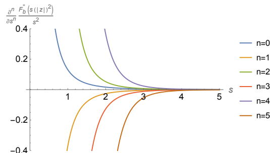
Figure 2. The function \frac{F_b''(s|z|^2)}{s^2} and its first five derivatives, evaluated at position z = i, \bar{z} = -i . The derivatives have alternating signs.
