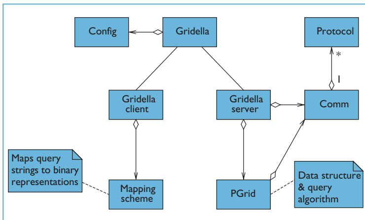
Figure 8. Gridella core system components. The Gridella client provides user-related functionality, while the server handles data management and communication.
