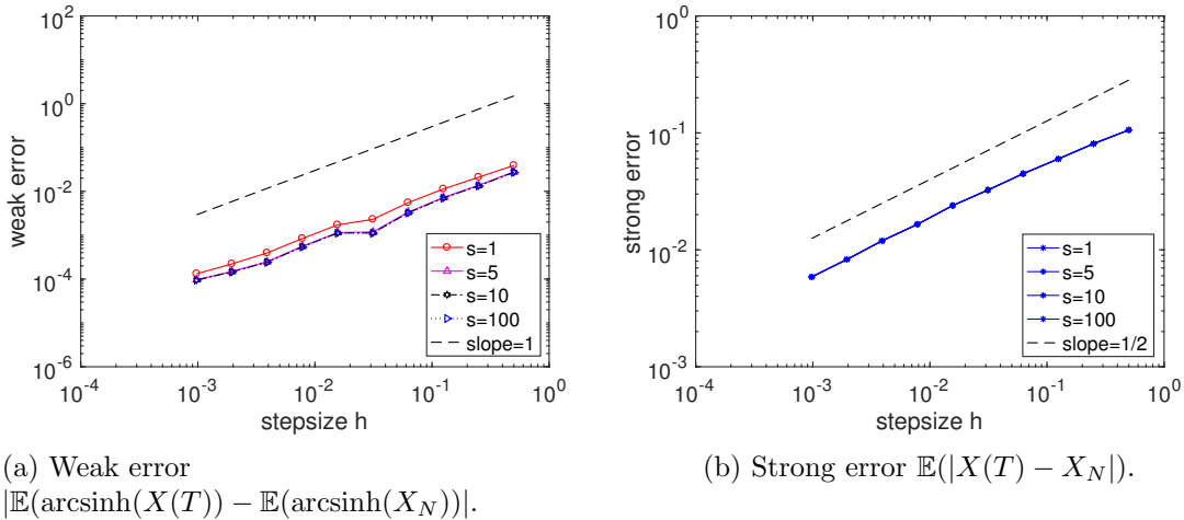
Figure 4: Nonlinear problem (51). Strong and weak convergence plots using SK-ROCK with final time T = 1 , stepsizes h = 2^{-p} , p = 1..10 , 10^4 samples and number of stages s = 1, 5, 10, 100 .
