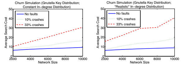
(a) Search performance under churn of Oscar with constant in-degree distribution (b) Search performance under churn of Oscar with “realistic” in-degree distribution
