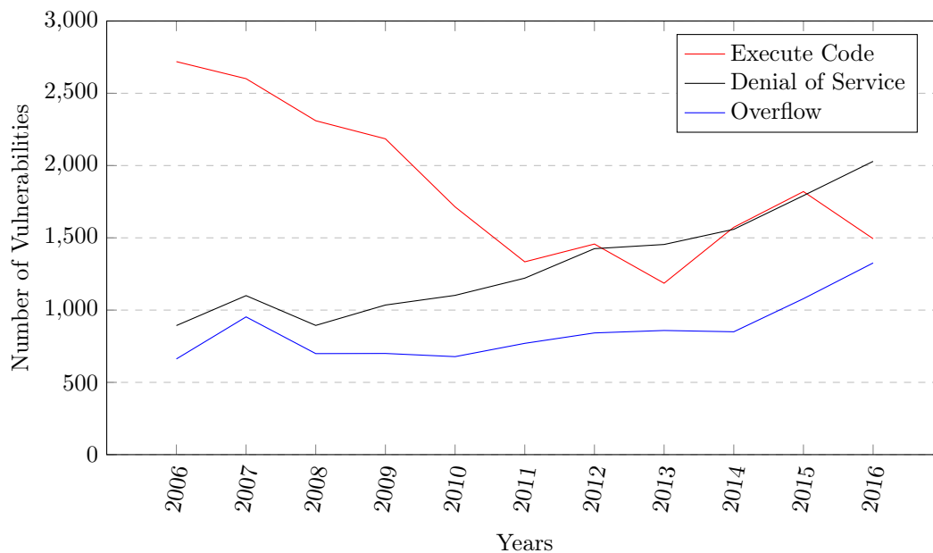
Figure 2: The 3 most frequent categories of bugs in the last 10 years. Source: [23]
