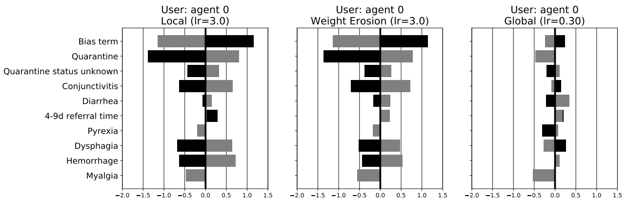
Figure 2: Parameters of the models in Figure 1 (left).
