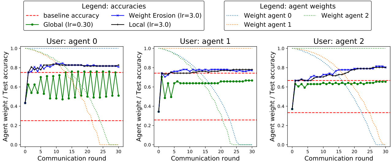
Figure 5: Predicting Ebola infection with AGE_SOME split. The Ebola data set is split across 3 agents by age group:
