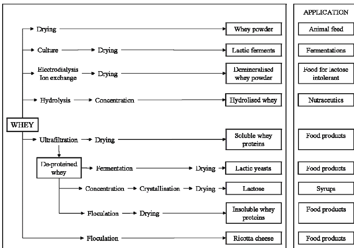
Figure 2. Valorization possibilities of whey.
