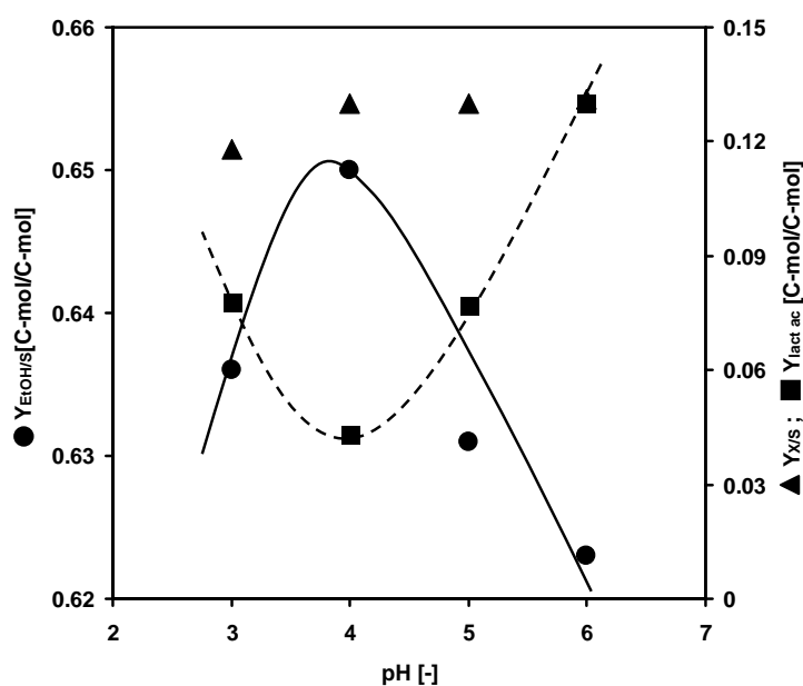
Figure 1. Dependency of ethanol performance parameters on pH for the mixed-culture CEKI, composed of K. marxianus (S1), I. orientalis (S2) and E. faecalis (S3). These cultures were performed at 30°C in 250 mL shake-flasks.
