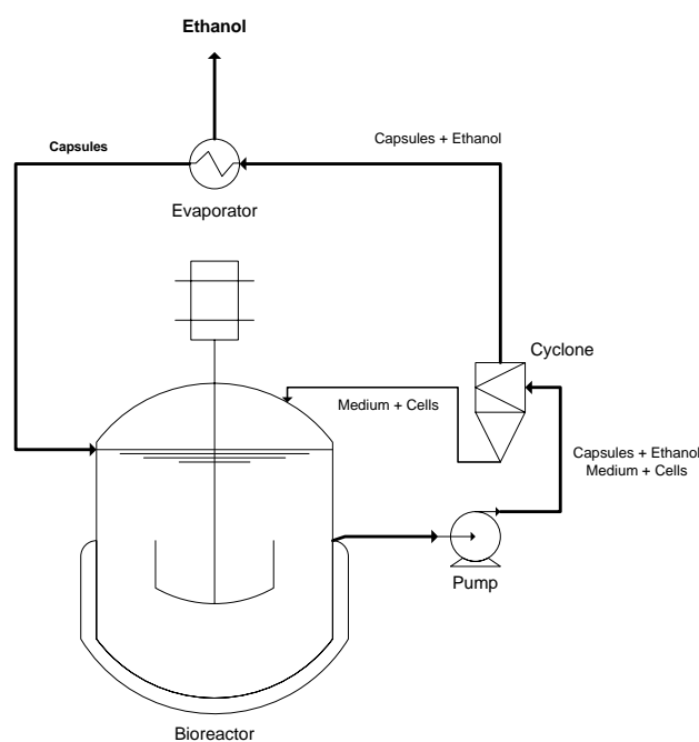
Figure 2. Flow chart of ethanol recovery from an encapsulated organic phase. The capsules are separated from the culture broth by a cyclone and heated to recover ethanol. Ethanol-free capsules are then recycled.
