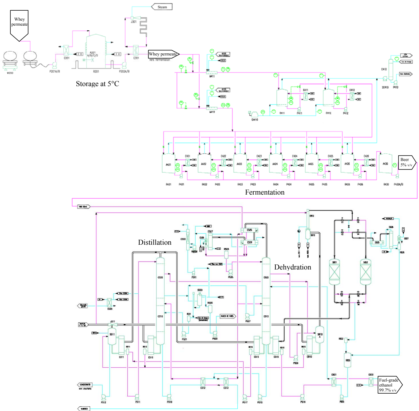
Figure 1. Process flowsheet of a centralized ethanol production plant from concentrated whey permeate. The whey permeate is refrigerated and stored at 5°C then feeds the fermentors, where a 5% v/v beer is produced. Successive distillation and dehydration produce fuel-grade ethanol at the end of the process [14].
