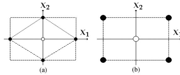
Figure 1. Comparison of the experimental surface covered by (a) the “one factor at a time” method and (b) the corresponding design of experiment model.
