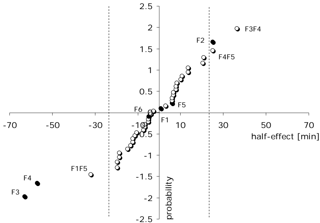
Figure 4. Plot of the normal half-effects on lag phase, where F1 is the biomass concentration, F2 the initial biomass concentration, F3 the type of sugar, F4 the culture mode, F5 the initial sugar concentration and F6 the temperature. Two levels were tested for each factor.
