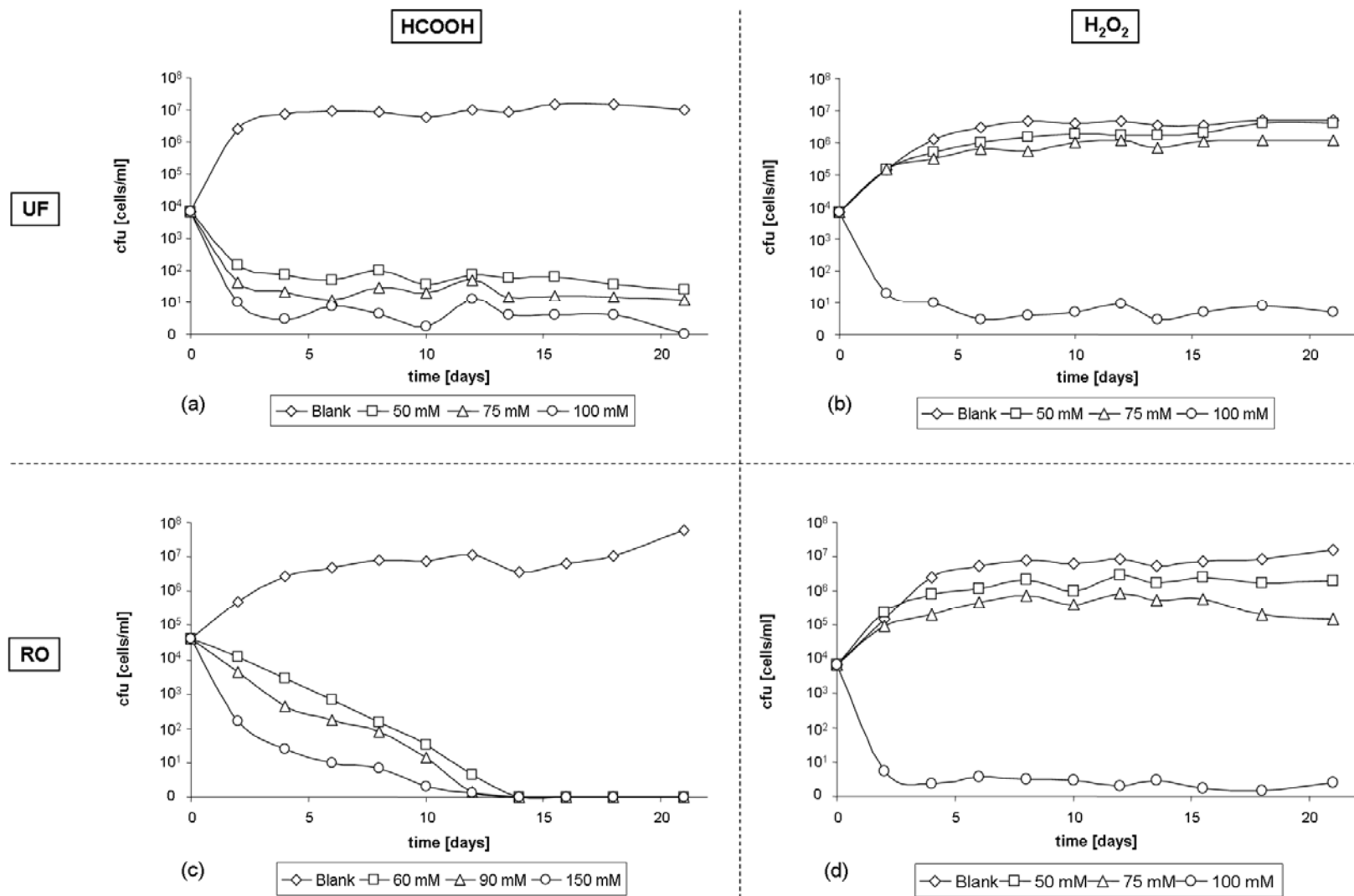
Figure 2. Bacterial cell numbers in (a) ultra-filtrated (UF) when permeate stabilized by formic acid at 25°C (b) UF when permeate stabilized by hydrogen peroxide at 25°C (c) reverse-osmosed (RO) treated when retentate stabilized by formic acid at 25°C (d) RO when retentate stabilized by hydrogen peroxide at 25°C. Cell density was measured as colony forming units after incubation on agar plate-count medium for 48h at 37°C.
