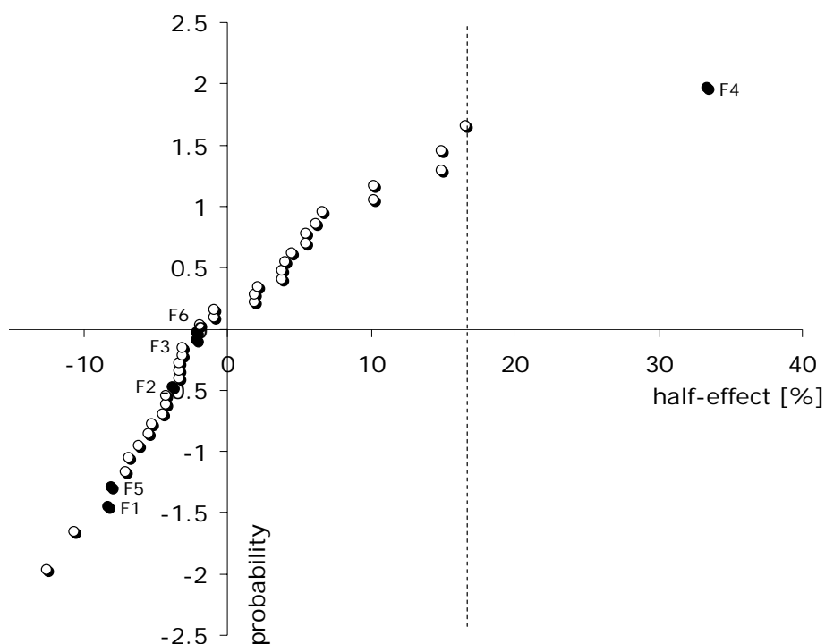
Figure 5. Plot of the normal half-effects on specific growth rate, where F1 is the biomass concentration, F2 the initial biomass concentration, F3 the type of sugar, F4 the culture mode, F5 the initial sugar concentration and F6 the temperature. Two levels were tested for each factor.
