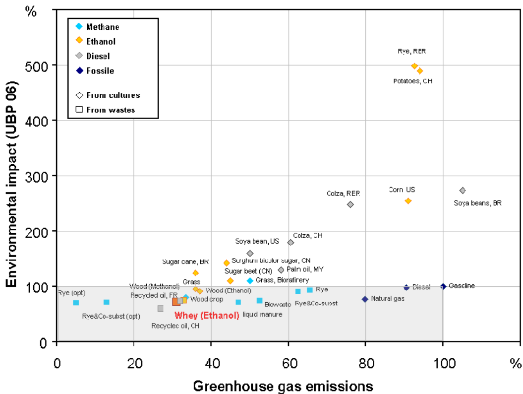
Figure 3. Two dimension representation of greenhouse gas emissions and overall environmental impact modeled with UBP 06 methodology [28]. Comparison is given to gasoline used as reference. Grey area shows the domain in which lower emissions and land damages compared to gasoline are achieved.
