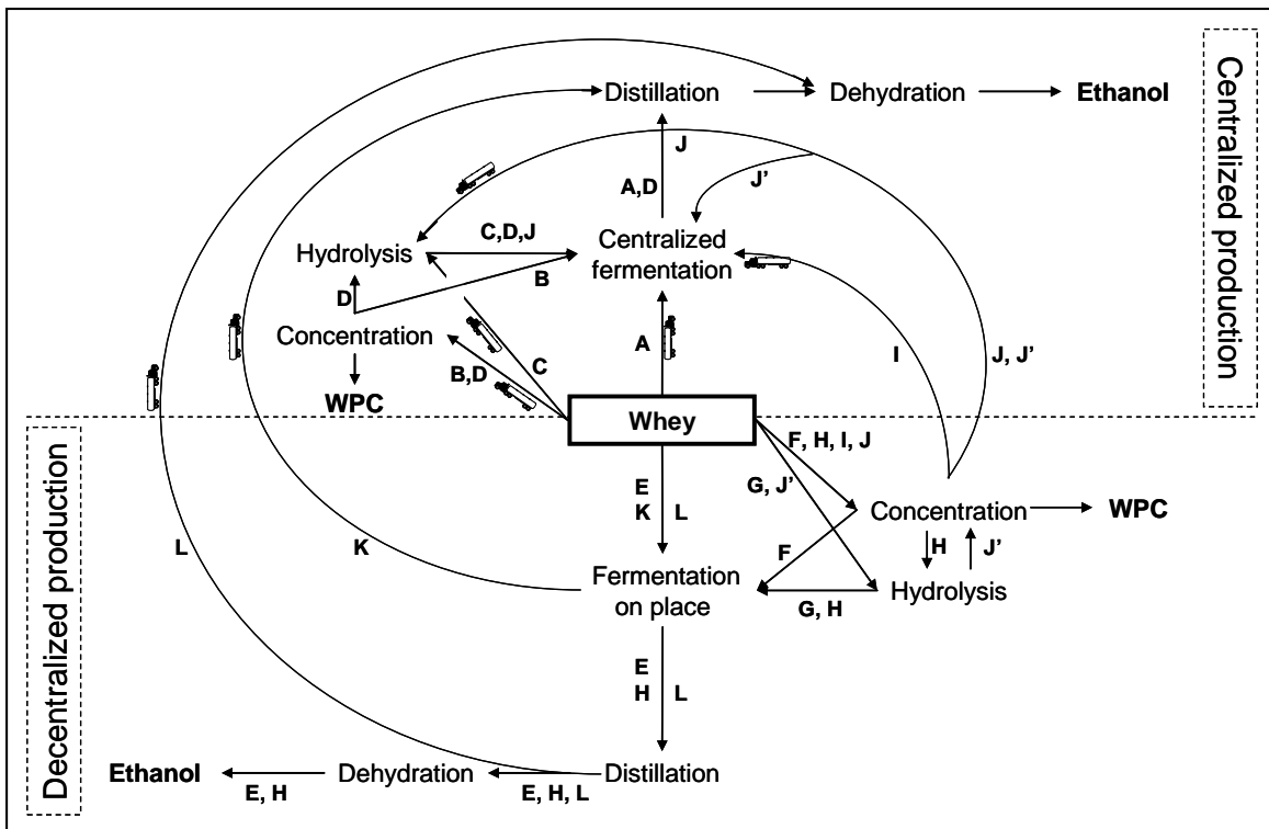
Figure 2. Possible ethanol production pathways from whey in either centralized, decentralized and hybrid production strategies. Scenarios A to D are possible totally centralized production pathways, where ethanol is produced in a unique common production plant; while scenarios E to H represent totally decentralized strategies, where ethanol is directly produced at the whey production site. Scenarios I to L depict the possible hybrid possibilities to produced ethanol, where part of the operating steps are first made at the production site than in a centralized production plant.
