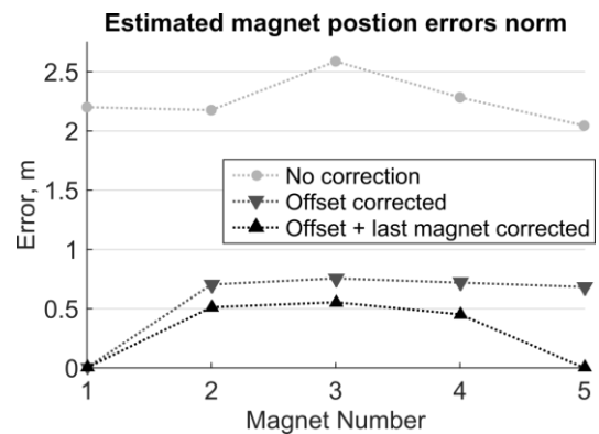
Figure 3: Total distance between estimated and true magnet position.
