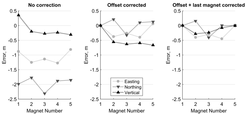
Figure 2: Error between estimated and true magnet position for each scenario.
