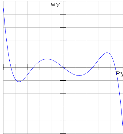
Figure 5. Ray-fan plot for a wavelength of 6 \mu\text{m} . The horizontal axis is the ray position in the pupil. It ranges from -1 to 1 mm. The full aperture corresponds to an NA of 0.87. The vertical axis is the ray divergence in milliradian. It ranges from -20 to 20 mrad.
