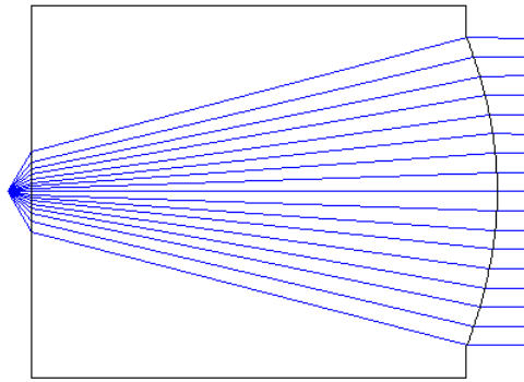
Figure 3. Schematic drawing of the collimating lens with a thickness of 3.0 mm and an aperture of 2.0 mm. The design benefit from the high refractive index of silicon.
