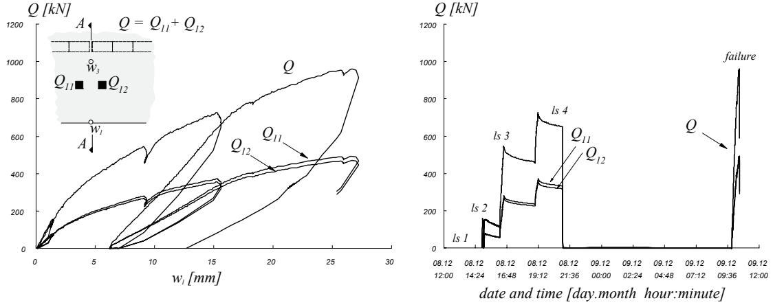
Figure A-4.19: Test DR2-a: Load history and load-deflection curve
