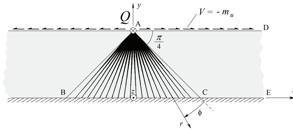
a) Lower bound solution
