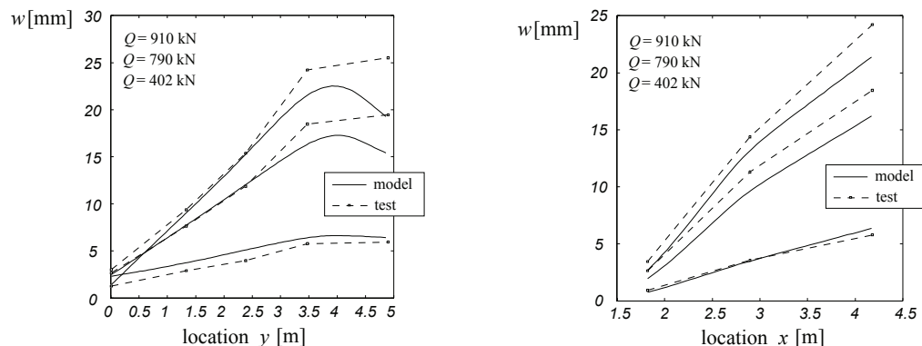
a) Along x = 4.18 m
