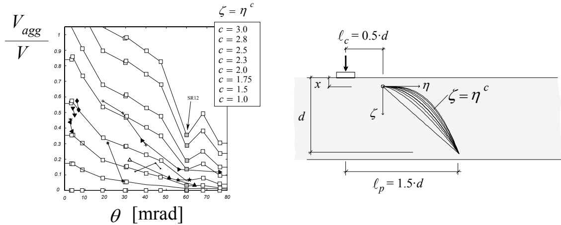
Figure 4.25: Sensitivity analysis on the form of the critical shear crack ( \zeta = \eta^c , \ell_c = 0.5 \cdot d , \ell_p = 1.5 \cdot d ) and comparison with measured values
