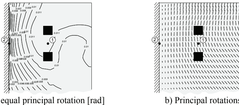
a) Lines of equal principal rotation [rad] b) Principal rotations Figure 5.32: Test DRI-b: location of points for calculation of the rotation \theta (from non linear analysis at Q=1025 kN)
