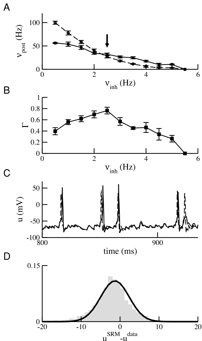
FIG. 10. Conductance injection. A: mean firing rate \nu_{\text{post}} of the SRM (solid line with squares) compared to that of the full model (dashed line with circles). Excitatory discharge frequency is kept constant at \nu_{\text{exc}} = 0.3 Hz, whereas we vary the inhibitory discharge frequency between 0.5 and 5.5 Hz. Each plotted symbol gives the mean computed over 5 spike trains of 1 s each with 1 SD (error bars). Arrow highlights the stimulation paradigm used for extraction of \varepsilon -kernels and optimization of the threshold. B: coincidence factor \Gamma . All the rest as in A. C: spike train of the SRM model (dashed line) is compared to that of the full fast-spiking neuron model (solid line; \nu_{\text{exc}} = 0.3 Hz and \nu_{\text{inh}} = 2.5 Hz). D: normalized histogram of the error in prediction of the subthreshold membrane voltage bin after bin for the same spike train as in C (light gray area). Fitted Gaussian distribution with \chi^2 = 0.001 ; mean = -1.3 mV, and SD = 3.7 mV (solid line).
