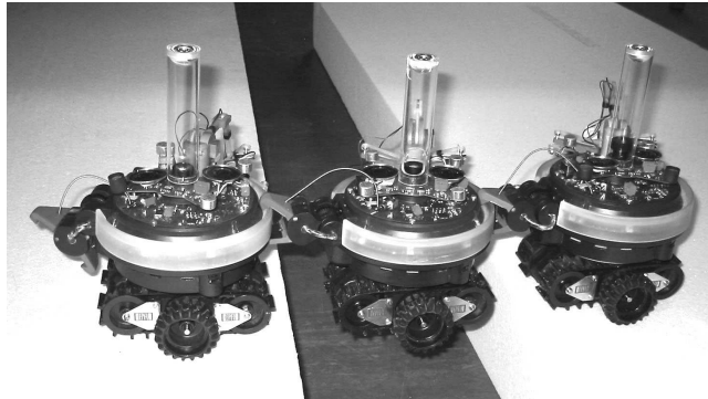
Fig. 3. Three s-bots passing a gap in swarm-bot configuration.
