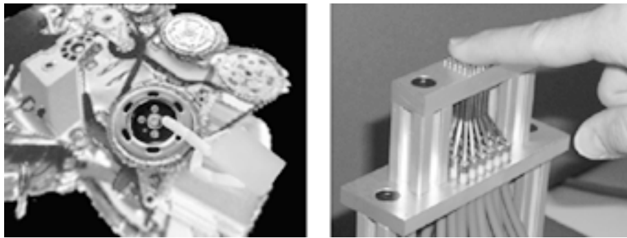
Figure 2. Tactile exploration of parts of a virtual car engine prototype.
