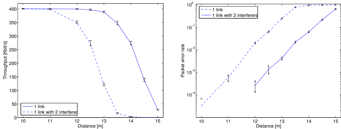
(a) Saturation throughput versus link distance with channel code rate 8/11. (b) Packet error rate versus link distance with channel code rate 8/11.
