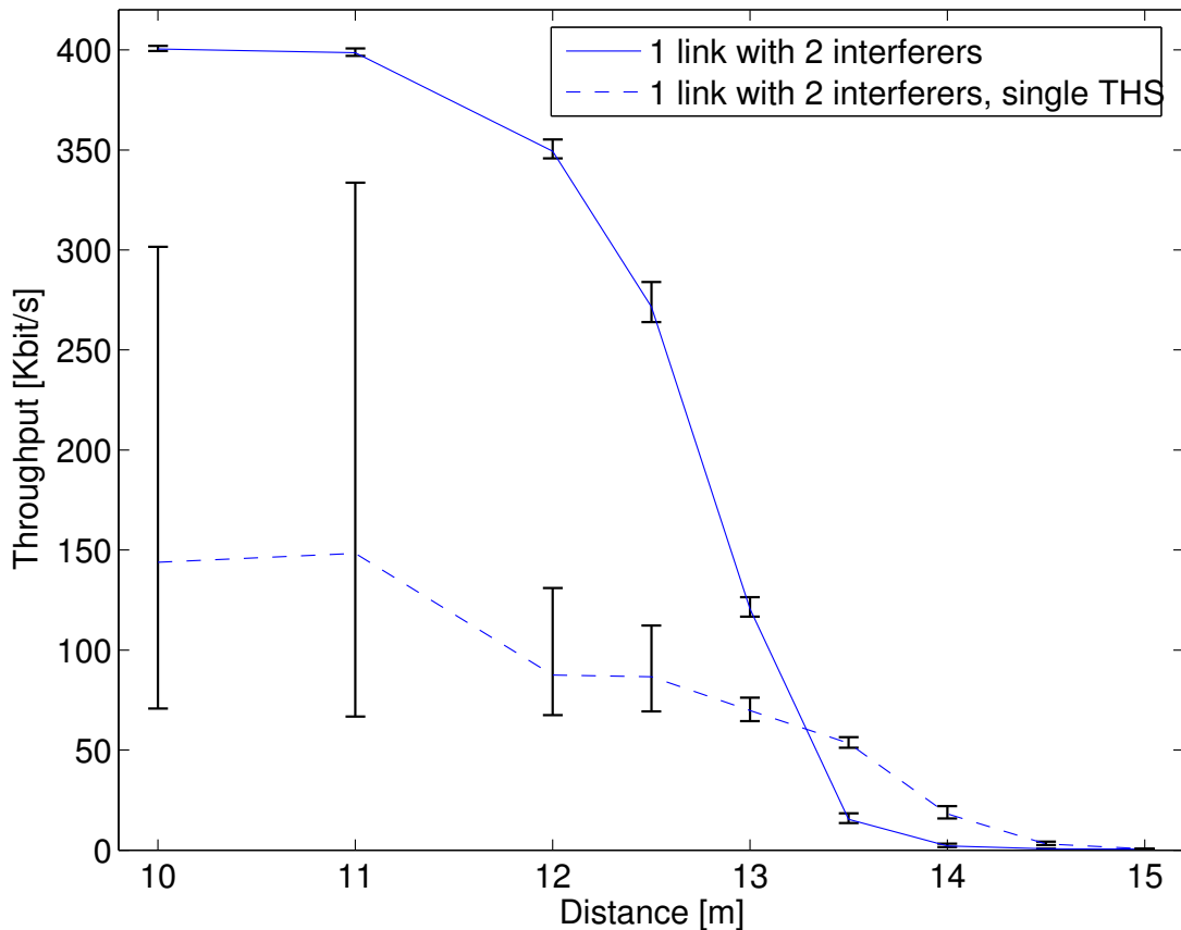
Fig. 4. Saturation throughput of the link S_0 to D_0 versus the link distance L with channel code rate 8/11. The topology is scenario 2. Using a single time-hopping sequence (dashed curve) in the network decreases the throughput compared to private time-hopping sequences (plain curve). Indeed, in this case, the nodes can acquire packets not sent to them.
