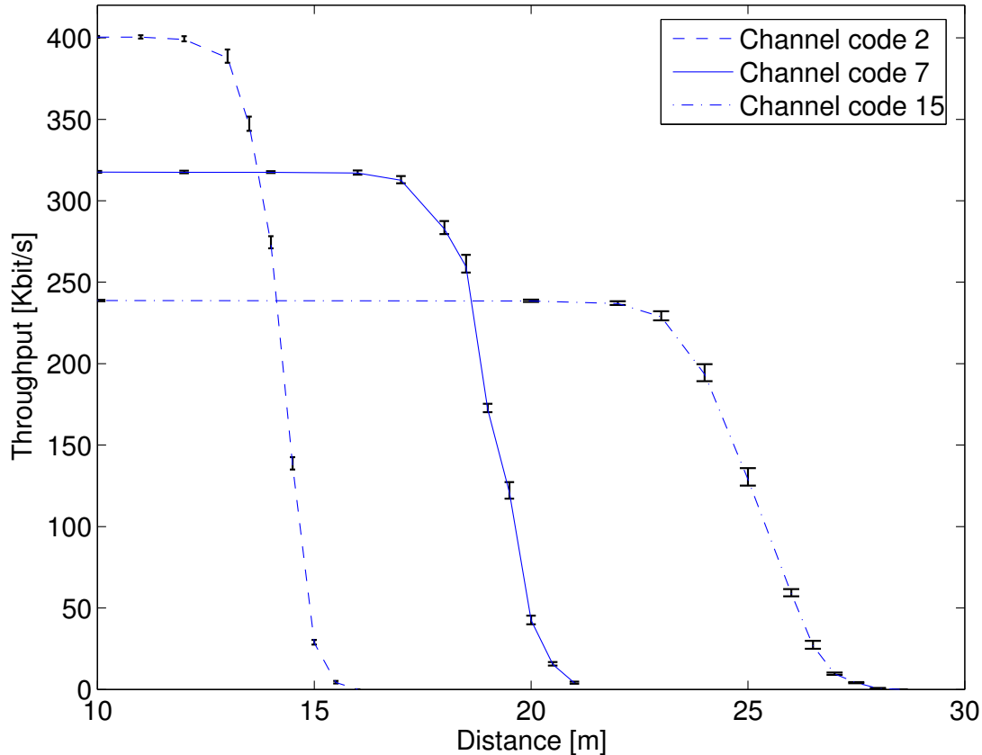
Fig. 2. Saturation throughput of the link S_0 to D_0 versus the link distance L for three different channel code rates. The topology is scenario 1. Due to the error model, the throughput smoothly decreases with the distance.
