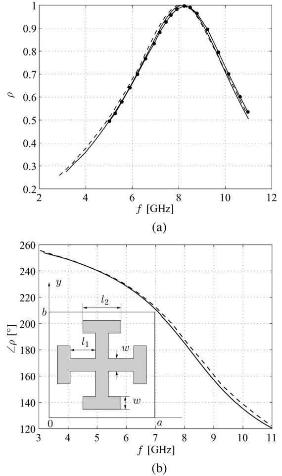
Fig. 4. (a) Magnitude and (b) phase of the reflection coefficient as a function of frequency for a normal incidence TE_{m0} illumination. Results obtained using the presented theory are denoted via solid lines, the values taken from [1] are denoted via dashed lines, and the values taken from [10] are denoted via circles. The inset shows a unit cell of the freestanding array of conducting patches in the shape of a Jerusalem cross. Dimensions are in millimeters: w = 1.9 , l_1 = 3.8 , l_2 = 5.7 , a_1 = a_2 = 15.2 .
