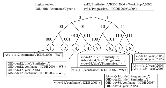
Figure 2: Example tuples stored in P-Grid
