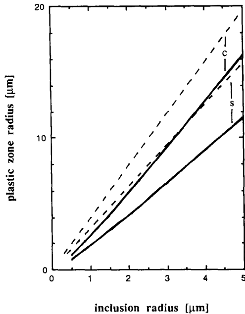
Fig. 10. Plastic zone radius around a SiC cylinder ( c ) and sphere ( s ) in a 99.5% aluminium matrix after a temperature change of 200 K. Materials constants are listed in Table 1. Full curves: strain-hardening matrix [equation (12)]. Dotted curves: non strain-hardening matrix [equation (6)].
