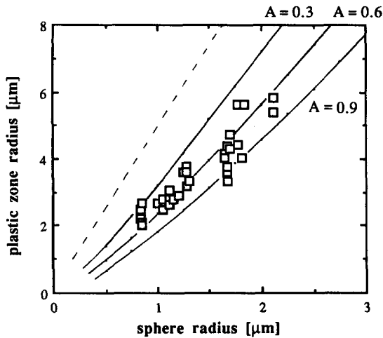
Fig. 13. Radius of plastic zone surrounding a sphere in an AgCl matrix as a function of the radius of the corresponding sphere. Squares: experimental data. Solid curves: strain-hardening matrix with different values of [equation (12b)]. Dashed curve: nonstrain-hardening matrix [equation (6b)].
