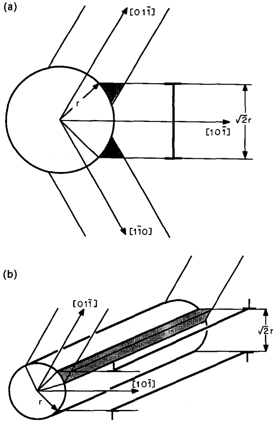
Fig. 9. (a, b) Schematic of prismatic dislocation loops punched in the \langle 110 \rangle directions of a f.c.c. lattice from a sphere (a) and a cylinder (b). The shaded volumes represent the intersection of adjacent glide systems.
