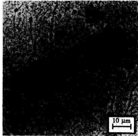
Fig. 7. Peanut-shaped plastic zone around an alumina fiber embedded in AgCl.
