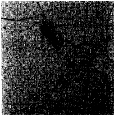
Fig. 6. Decorated rows of prismatic loops punched from a short alumina fiber in an AgCl matrix. After bursting through a subgrain boundary (dark continuous line), the loops change orientation in the second subgrain. Partially resolved dislocation tangles are also decorated around the fiber.
