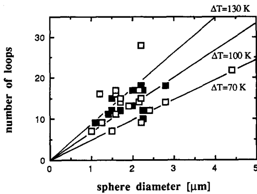
Fig. 11. Total number of prismatic dislocations loops punched by glass spheres in AgCl as a function of the sphere diameter. Open squares: single row of loops. Solid squares: double rows of loops. Lines: calculations from equation (18) for different values of \Delta T .
