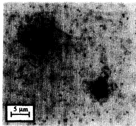
Fig. 4. Glass spheres in AgCl matrix surrounded by tangled, decorated dislocations in a plastic zone forming lobes.
