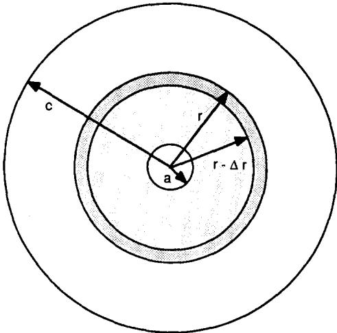
Fig. 8. Fictitious hole expanded from zero radius to radius a producing a plastic zone of radius c and a matrix displacement of \Delta r at the surface of the inclusion of radius r . Cylindrical or spherical case.
