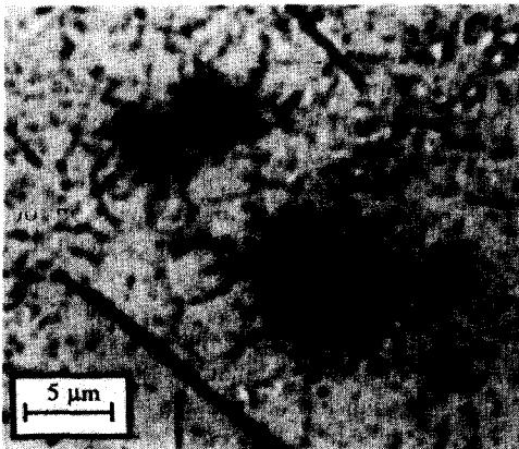
Fig. 2. Unresolved dislocations forming a spherical plastic zone around glass spheres embedded in AgCl.
