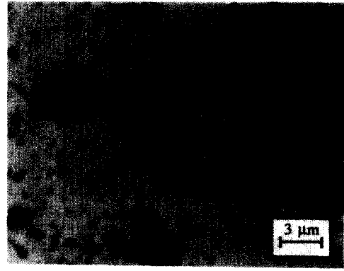
Fig. 3. Glass sphere in AgCl matrix surrounded by an irregular zone of unresolved, decorated dislocations and having emitted prismatic loops.
