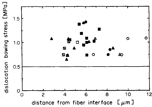
Fig. 12. Stress of pinned dislocations as calculated from equation (12) in the plastic zone surrounding alumina fibers in an AgCl matrix (see Fig. 5) as a function of radial distance from the interface. The various symbols represent different fibers. The lower horizontal line is the value of the microyield stress in shear as measured by other investigators [67–68].
