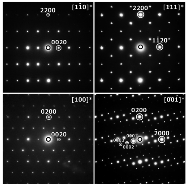
Figure 3. [110]*, [111]*, [100]*, and [001]* ED patterns of the incommensurately modulated KNd(MoO 4 ) 2 phase.
