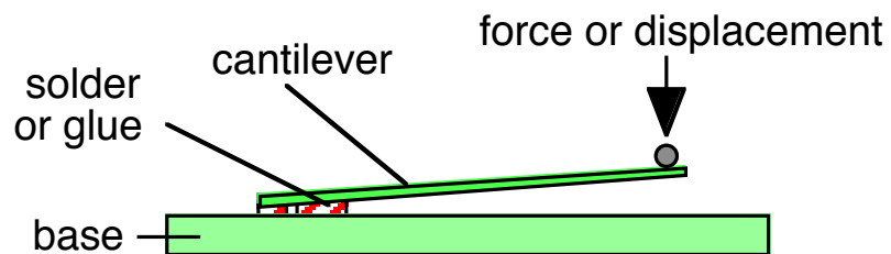
sensor schematic
