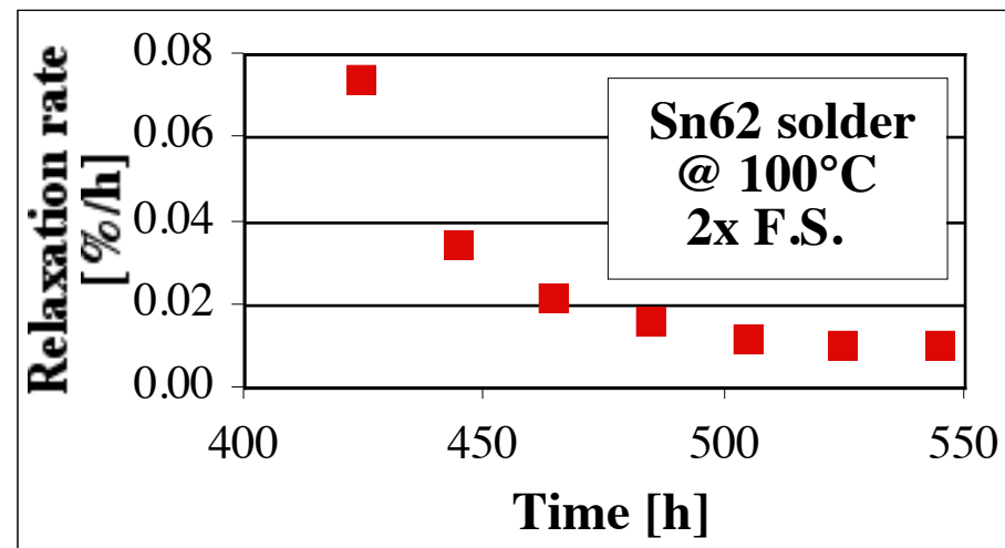
typical displacement sensor relaxation curve
