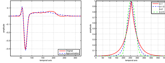
Fig. 1. Left: QRST VA complex and its approximation using just 3 atoms. Right: Effect of \beta on the GGF (see Eq. (5)).
