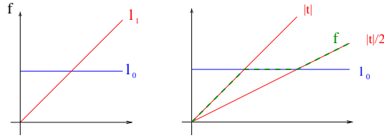
Figure 1: (a) The “nice” functions f_0(t) and f_1(t) corresponding to the \ell^0 and the \ell^1 norm (b) An “exotic” sparsity measure, based on a mix of the \ell^0 and \ell^1 measures plotted in (a).
