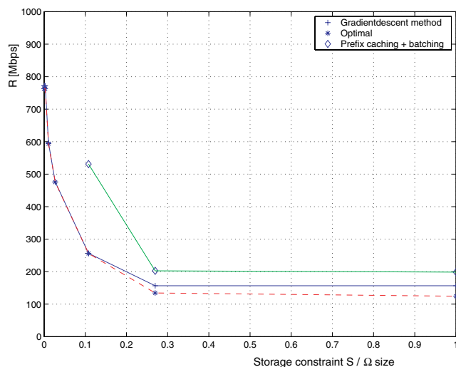
Figure 9: Aggregate backbone rate vs. proxy storage capacity for a heterogeneous set of A = 50 media assets, \Delta = 2 seconds, d = 3 seconds and B = 1.33 Gbps using Algorithm A1 and the optimal. The simpler method where N_\omega = 0 for all \omega \in \Omega (pure prefix batching) is also shown.
