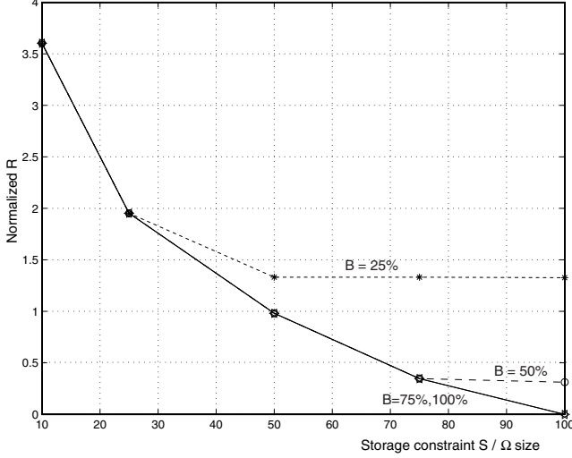
Figure 3: Normalized backbone rate vs. cached prefix size (when the bandwidth out of the proxy is constrained).
