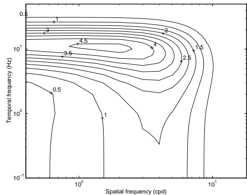
Figure 6. Contour plot of the estimated spatio-temporal CSF.
