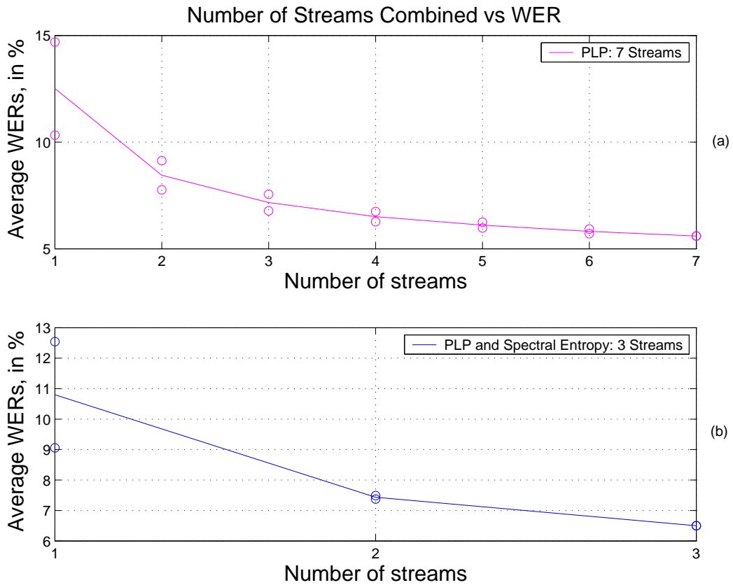
Figure 6.1. Performance of oracle in % WERs for multi-stream combination. (a) The streams are all possible combinations of the static PLP features and their first and second order time derivatives (7 streams). Out of 7 streams, 'n' streams were used for combination, 'n' varying from 1 to 7. (b) The streams considered for combination were PLP features with first and second order time derivatives, spectral entropy features derived from 24-Mel band with their first and second order time derivatives and concatenation of the two features (3 streams). 'n' varied from 1 to 3.
