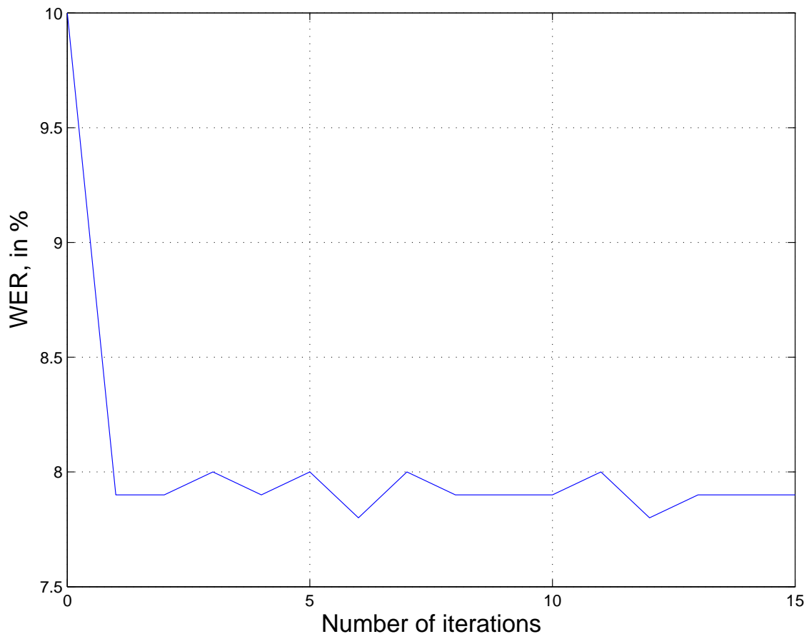
Figure 6.5. Embedded hybrid training for a single-stream (baseline PLP features): 'number of iterations' vs WER. 0 th iteration has hand-labelled segmentation for training the MLP. The first iteration gives the maximum improvement.
