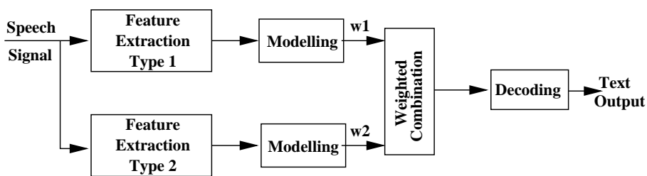
Figure 3.2. Posterior (or likelihood) combination: Different feature representations are obtained from the speech signal and modelled separately. The outputs of the models (either posteriors or likelihoods) are weighted and combined. The combined outputs are decoded.
