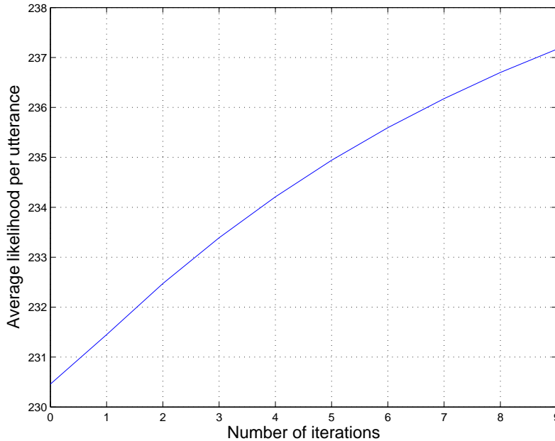
Figure 4.5. ML Weighting (Batch Mode): Evolution of average likelihood per utterance from one iteration to another.
