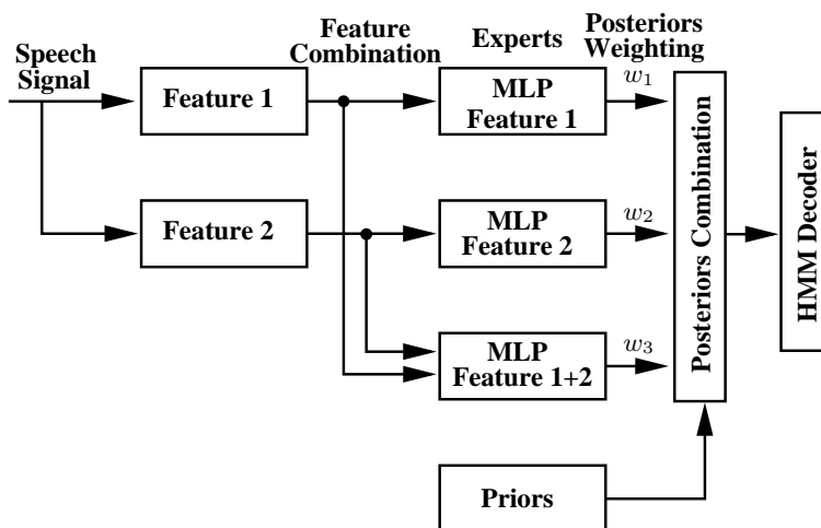
Figure 3.4. Full-combination multi-stream for a hybrid HMM/ANN system: All possible combinations of the two feature representations are treated as separate feature streams and an MLP is trained for each feature stream. The posteriors at the output of the MLPs are weighted and combined. The combined posteriors thus obtained are passed to an HMM decoder to generate text output.
