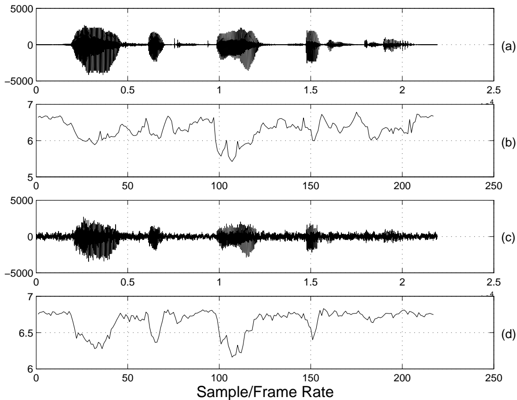
Figure 5.2. Entropy computed from the full-band spectrum. (a) A clean speech waveform from the Numbers95 database, (b) Spectral entropy contour for the clean speech waveform, (c) Speech waveform corrupted by factory noise at 6 dB SNR, and (d) Spectral entropy contour for the speech waveform corrupted by factory noise at 6 dB SNR. Factory noise is taken from the Noisex92 database and added to the clean speech waveform.
