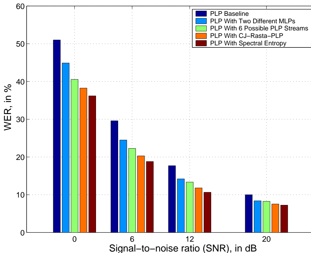
Figure 6.3. Complementarity of different multi-stream setups using oracle test. The oracle performance in % WERs is compared for: a) Same PLP baseline features with different MLP sizes, b) 6 possible PLP feature streams with baseline PLP features, c) CJRASTA-PLP features with baseline PLP features, and d) Spectral entropy features with baseline PLP features.
