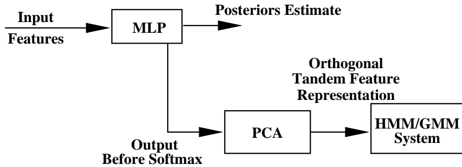
Figure 7.2. Tandem Linear Model: ‘Outputs before softmax’ from the MLP are decorrelated by PCA and used as features in a standard HMM/GMM system.
