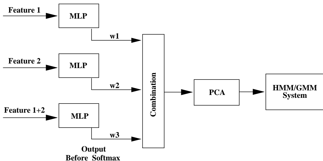
Figure 7.4. Multi-stream Linear Tandem: ‘Outputs before softmax’ from different MLPs are weighted and combined. The combined output undergoes PCA before being fed as features into an HMM/GMM system.
