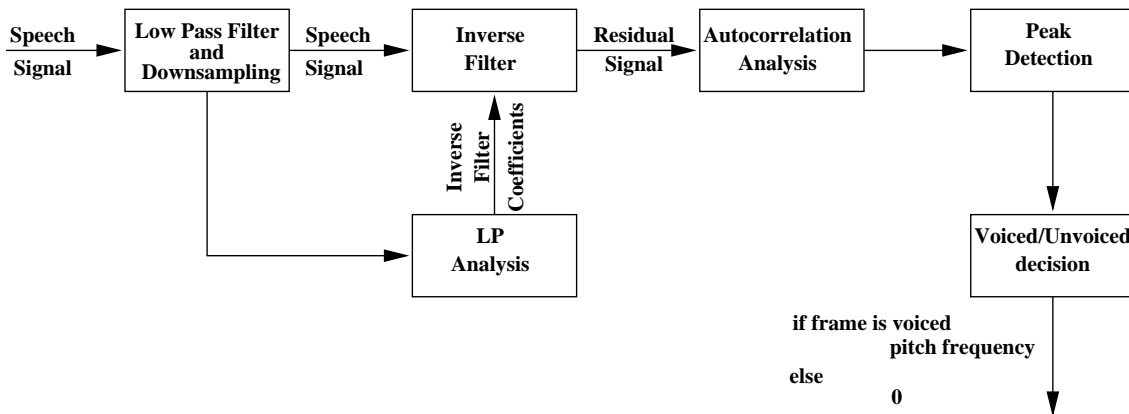
Figure 5.1. SIFT algorithm for extracting pitch frequency.
