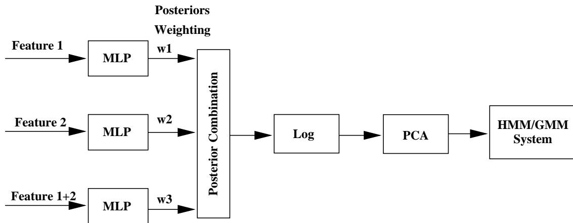
Figure 7.3. Multi-stream Softmax Tandem: Posteriors from different MLPs are weighted and combined. The combined output undergoes log scaling followed by PCA before being fed as features into an HMM/GMM system.
