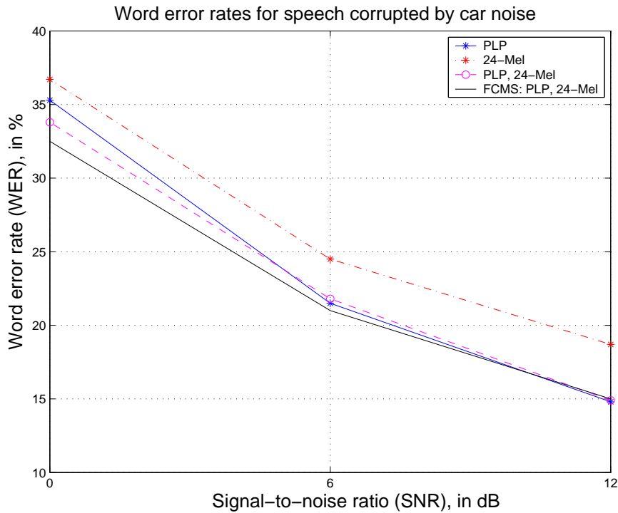
Figure 5.4. Performance in % WER of different feature streams for a hybrid system for car noise at different SNRs. The plot shows baseline PLP (-*-), spectral entropy features derived from overlapping sub-bands defined on a Mel scale (-*), spectral entropy features appended to the PLP features (-o-) and the two features in FCMS (—). Car noise is taken from the Noisex92 database and added to the utterances of the Numbers95 database at different SNRs.
