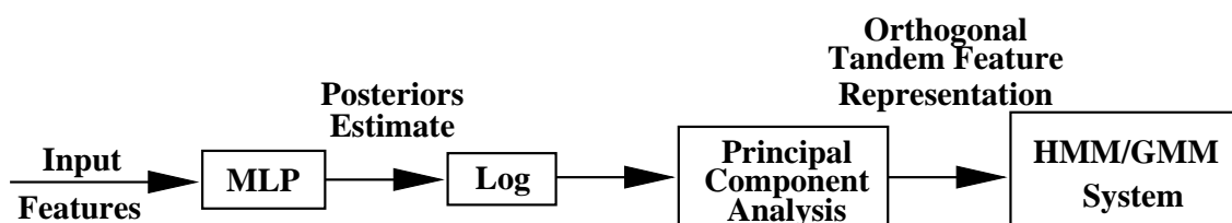
Figure 7.1. Tandem Posterior Model: Posteriors from the MLP are \log scaled and then decorrelated by PCA. The transformed posteriors are used as features in a standard HMM/GMM system (Hermansky et al., 1999).
