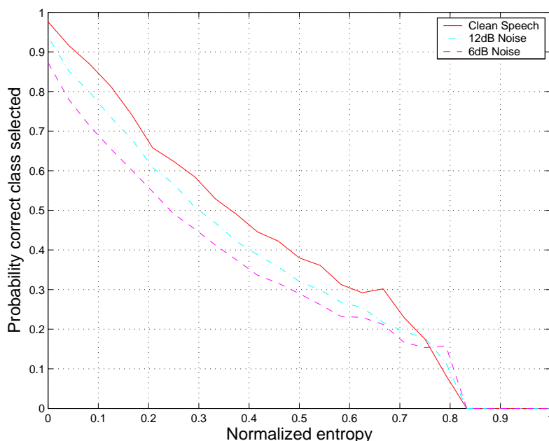
Figure 4.2. Plot of normalised entropy vs probability that the correct class is selected. The plot is for the MLP trained on clean PLP features and for the following test conditions: Clean (—), SNR12 (-.-) and SNR6 (- - -). The database for training and testing is Numbers95 and noise conditions are simulated by adding factory noise from the Noisex92 database to the test data.
