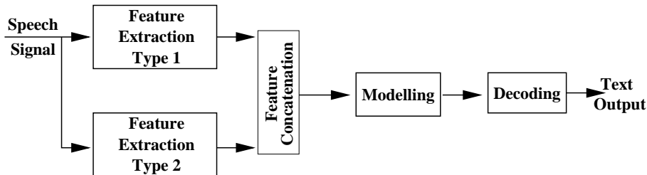
Figure 3.1. Feature combination: Different feature representations are obtained from the speech signal and appended (concatenated) to form a feature vector. The combined feature vector is modelled and decoded by the usual ASR system.
