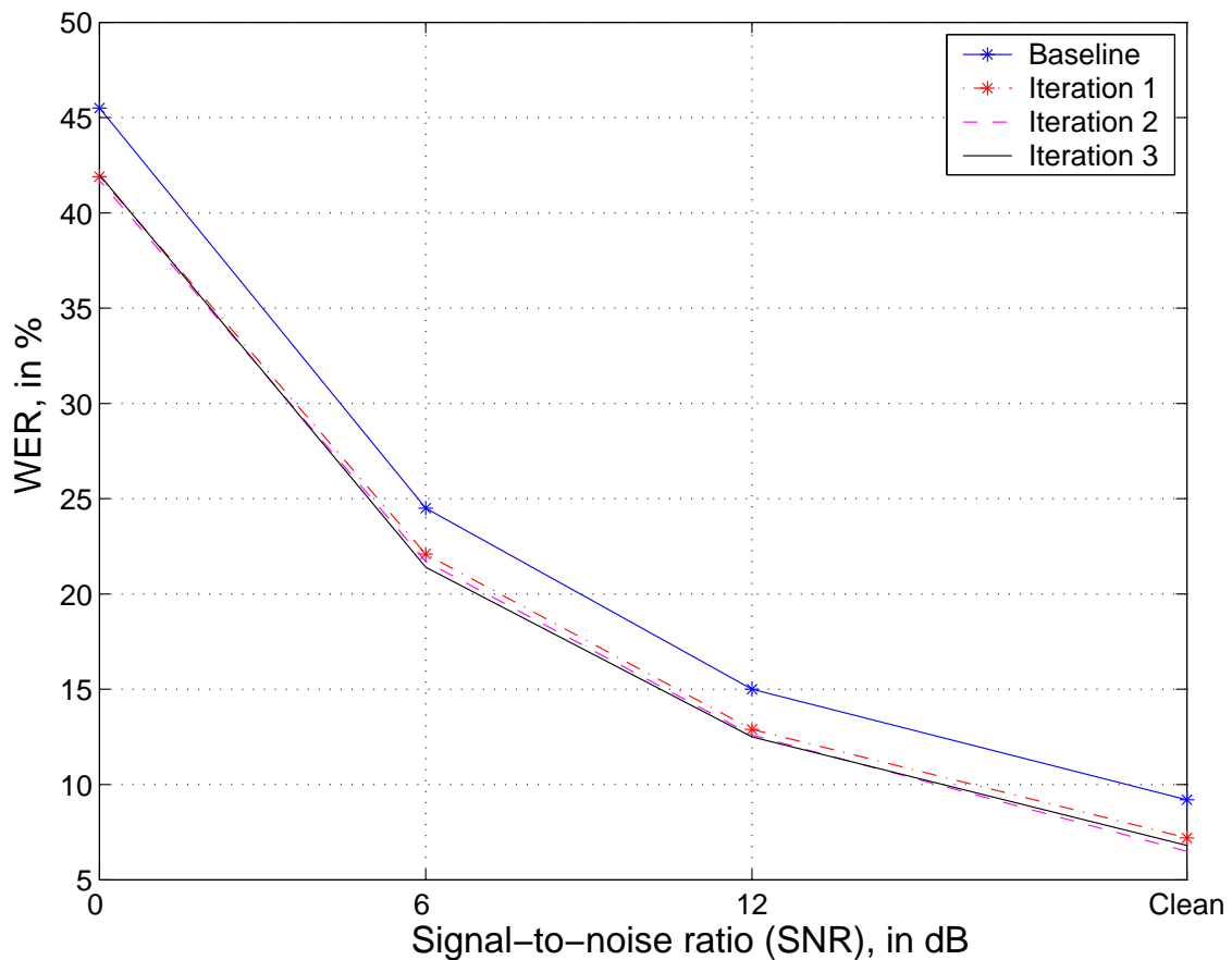
Figure 6.7. Embedded hybrid training for FCMS: Comparison of performance in % WER with training performed on hand-labelled segmentation and segmentation obtained by forced alignment after each iteration. The performance is compared for clean test condition (20 dB SNR) as well as noisy test conditions. Noise conditions are simulated by adding factory noise from the Noisex92 database to the utterances of the Numbers95 database at various SNRs.
