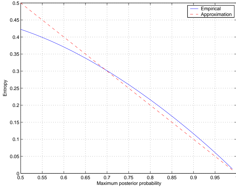
Figure 4.4. Relationship between maximum-posterior probability and entropy at the output of an MLP for number of classes ( K ) equal to 27. The MLP was trained on the Numbers95 database. Solid line (—) is the empirical relationship obtained from the data and dashed line (- -) is the relationship developed by the approximation of (4.15).
