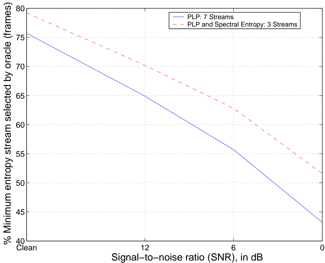
Figure 6.4. Number of times (in percentage of frames) oracle selected the stream with minimum entropy in the FCMS hybrid systems. The plot is for clean as well as noisy test conditions. Noise conditions are simulated by adding factory noise from the Noisex92 database to the utterances of the Numbers95 database at various SNRs. In the plot, clean speech condition is represented by 20 dB SNR.
