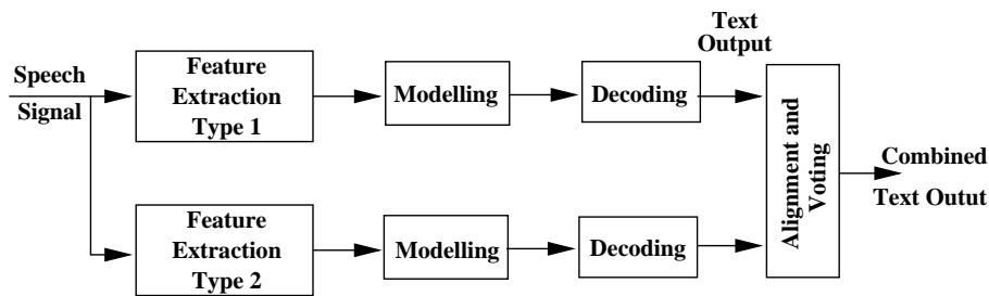
Figure 3.3. Decoder output combination: Different feature representations obtained from the speech signal are modelled and decoded separately by individual ASR systems. The decoded output (which is text) is combined with techniques such as majority voting to get the final text output.
