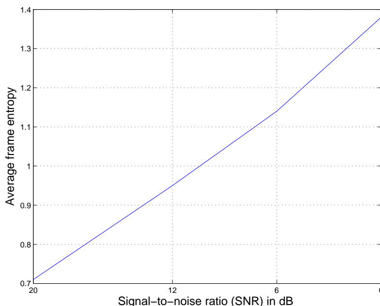
Figure 4.3. Change in average frame entropy at the output of an MLP with increase in noise-level at the input of the MLP. The MLP was trained on features extracted from clean speech and tested on features extracted from clean as well as noisy test utterances. The Numbers95 database was used for training and testing. Noise conditions were simulated by adding factory noise from the Noisex92 database at various SNRs to the clean speech. In the plot, the clean test condition is represented by 20 dB SNR.
