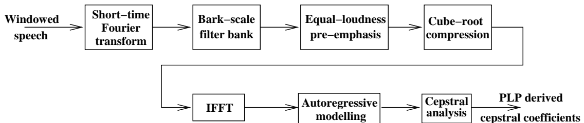
Figure 2.2. Extraction of PLP derived cepstral coefficients from short time windowed speech signal.
