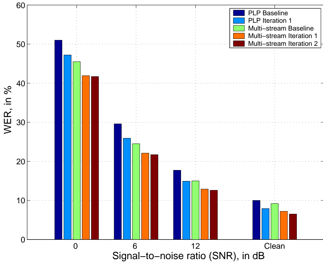
Figure 6.8. Performance in % WER for PLP features with hand segmentation, PLP features with segmentation obtained by forced alignment during embedded training (first iteration), PLP and spectral entropy features in FCMS with inverse entropy weighting and hand segmented labels, PLP and spectral entropy features in FCMS with segmentation obtained by forced alignment during embedded training (first two iterations). The performance is shown for clean test condition (20 dB SNR) as well as noisy test conditions. Noise conditions are simulated by adding factory noise from the Noisex92 database to the utterances of the Numbers95 database at various SNRs.
