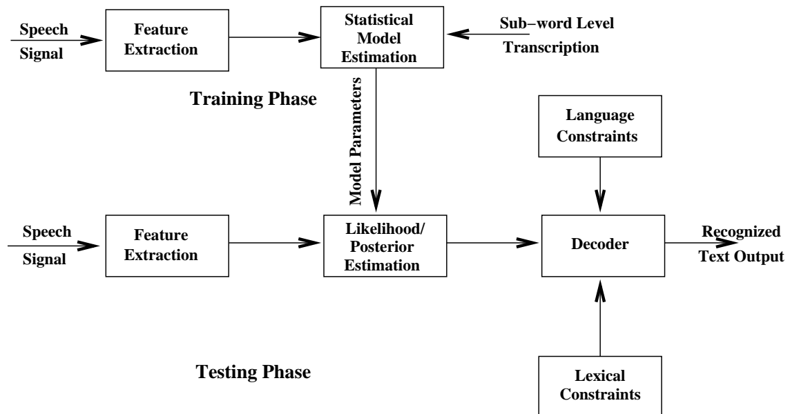
Figure 2.1. A standard speech recognition system with training and testing phases.
