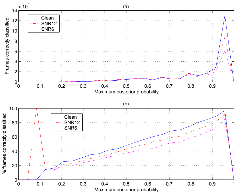
Figure 4.1. Empirical relationship between maximum-posterior probability at the output of an MLP and: (a) the number of frames correctly classified, (b) the percentage of frames correctly classified. The plot is for an MLP trained on clean PLP features and for the following test conditions: Clean (—), SNR12 (-.-) and SNR6 (- - -). The database for training and testing is Numbers95 and noise conditions are simulated by adding factory noise from the Noisex92 database.
