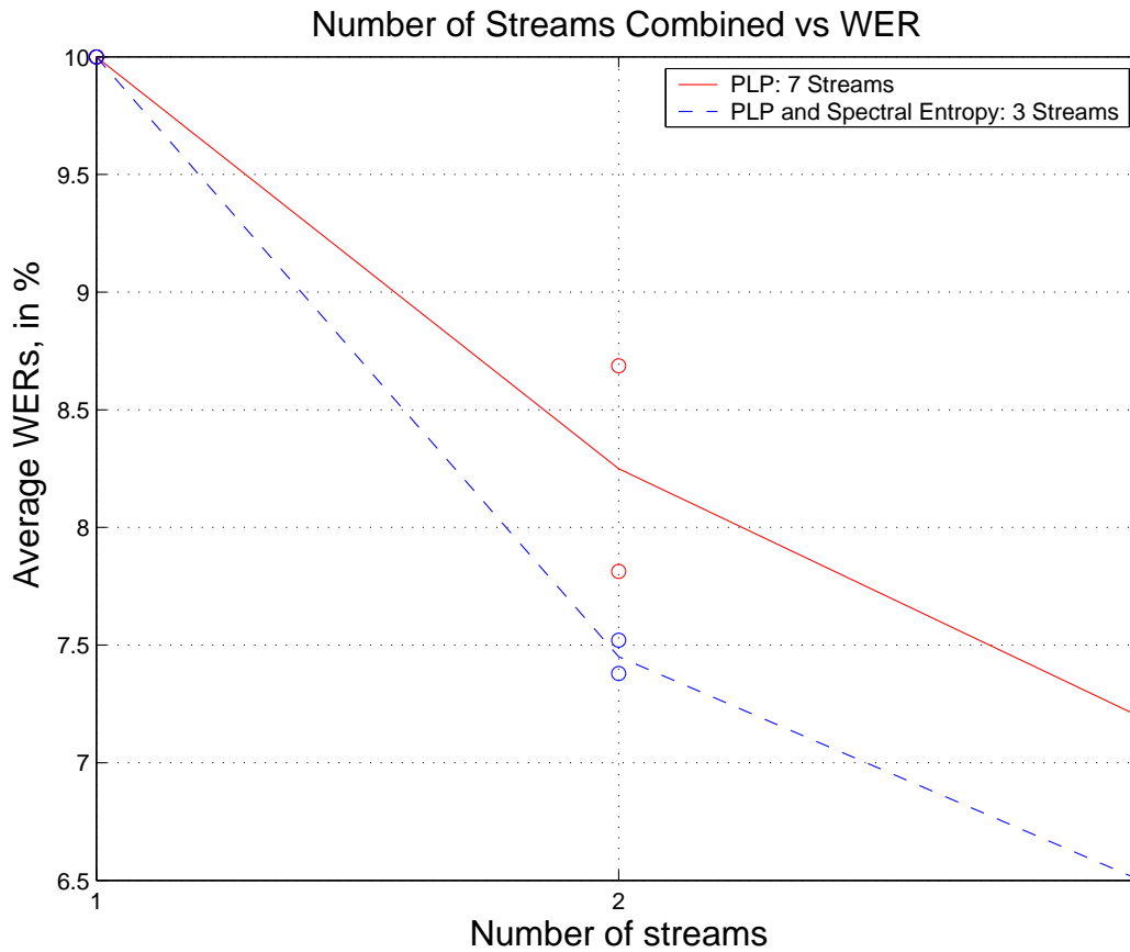
Figure 6.2. Oracle performance in % WERs to find out complementarity of streams used in multi-stream combination. The performance is compared for PLP features (static, delta and delta-delta) in FCMS (7 streams: —) and PLP features along with spectral entropy features in FCMS (3 streams: - - -)
