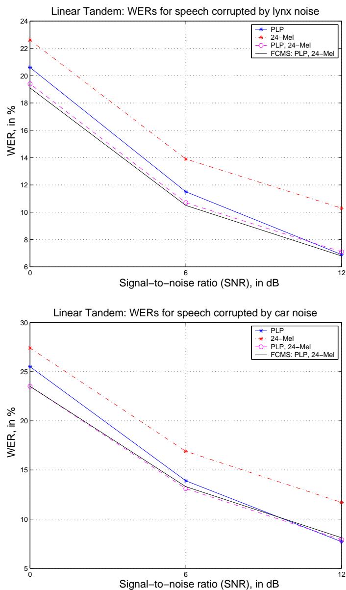
Figure 7.6. Multi-stream Linear Tandem (outputs before softmax): Plot of WERs for different feature streams for the Numbers95 database (Top): lynx noise added from the Noisex92 database at various SNRs, (Bottom): car noise added from the Noisex92 database at various SNRs. PLP features (-*-), spectral entropy features (-*.), the two features concatenated (-o-) and the two features in FCMS with inverse entropy weighting (—).
