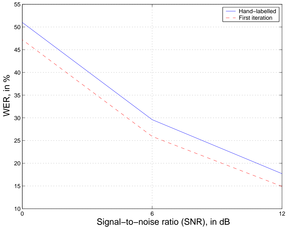
Figure 6.6. Embedded hybrid training for a single-stream (baseline PLP features): Comparison between WERs obtained by hand-labelled segmentation and with segmentation obtained by forced alignment (first iteration). Noise conditions are simulated by adding factory noise from the Noisex92 database to the utterances of the Numbers95 database at various SNRs.
