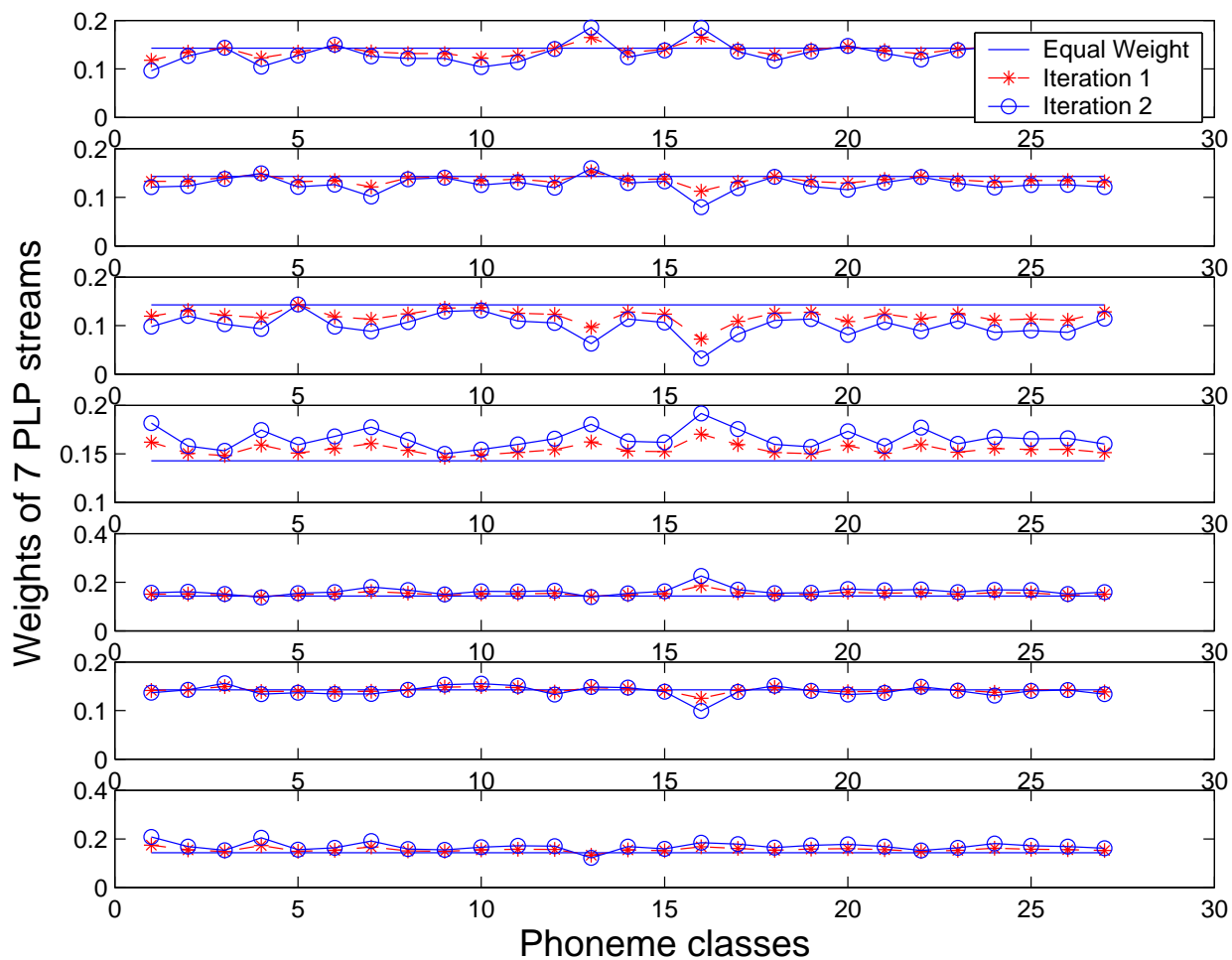
Figure 4.6. ML Weighting (Batch Mode): Evolution of weights for first three iterations.
