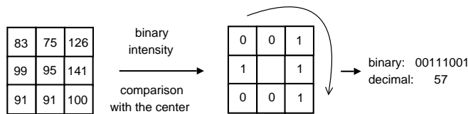
Figure 1: The LBP operator.
