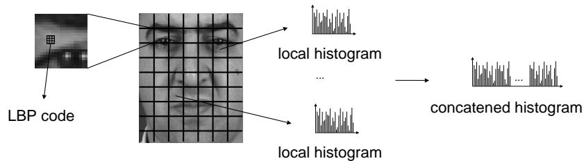
Figure 2: LBP face description with three levels of information: pixel level (LBP code), region level (local histogram), image level (concatened histogram).
