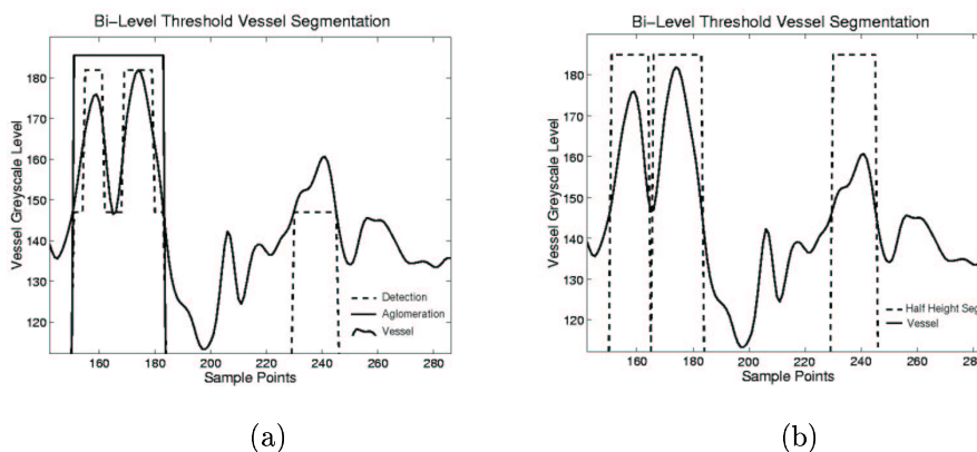
Figure 3: Bi-Level versus half height segmentation: (a) shows the results from the bi-level thresholding method developed in this work, (b) shows the result from a normal half-height thresholding method as presented in [9].
