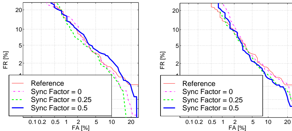
Figure 3 : Results for different sync factors ( \alpha ) with the joint likelihood approach. Independent training (left) vs. synch. alignment training (right). Silences are not removed
