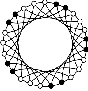
Fig. 1. Facet of C^1 : \sum_{v \in \circ} x_v + 2 \sum_{v \in \bullet} x_v \leq 6
