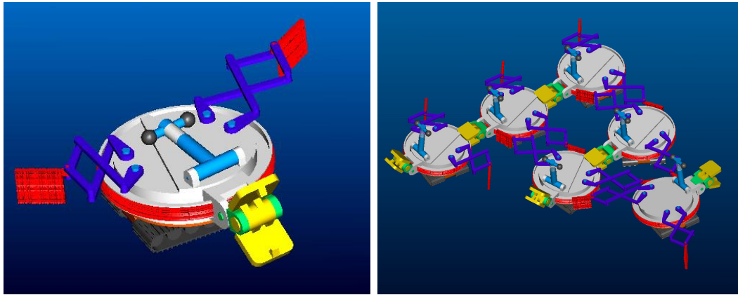
Figure 1: A graphic visualization of the first s-bot concept (left). The diameter of the main body is 110 mm. Several s-bots can self-assemble into a swarm-bot (right).
