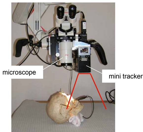
Fig.1: The Image-guided surgical microscope with mounted mini-tracker
