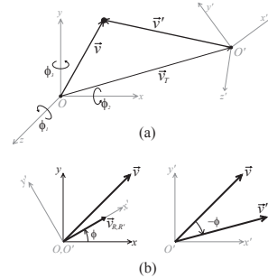
Figure 3: 3D FR transformations decomposed into three rotations and one translation at the origin (a). Rotation in a plane (b).
