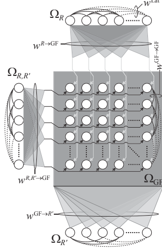
Figure 4: Network architecture.
