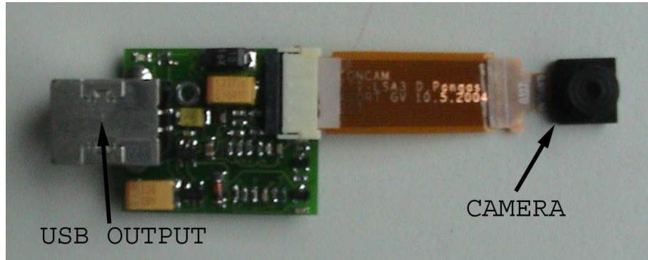
Figure 5: Camera module showed from above
