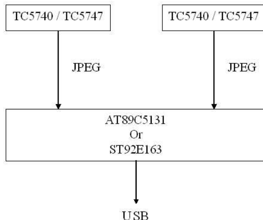
Figure 4: Solution using two TC574X cameras and a chip in order to have an USB output
