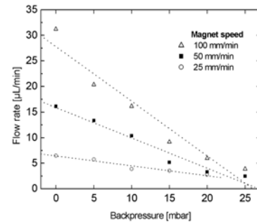
Fig. 3 : Pressure-flow characteristics of water for different speeds of the rare-earth magnet.
