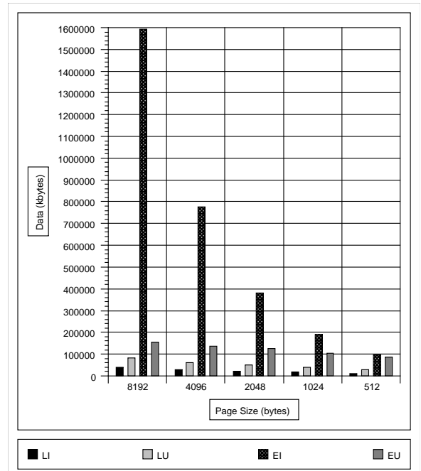
Figure 6 LocusRoute Data.
