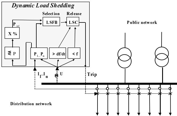
Figure 4: Dynamic Load Shedding for a Distribution Network
