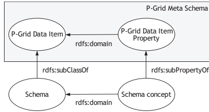
Fig. 3. Relations of a P-Grid custom schema to the P-Grid meta schema
