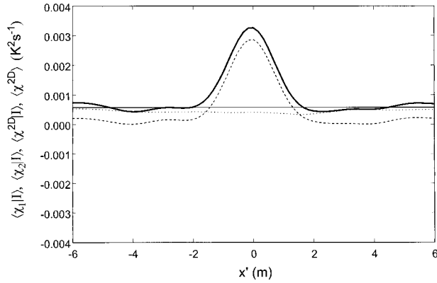
FIG. 10. Conditionally averaged surrogates of the SGS dissipation of temperature variance, under condition I ( \partial\theta/\partial t < -\sigma_{\text{ab}(\text{oi})} ), for measurement period U (unstable surface layer). Streamwise component \langle \chi_1 | I \rangle (dashed line), spanwise component \langle \chi_2 | I \rangle (dotted line), and 2D surrogate \langle \chi^{2D} | I \rangle (thick solid line). The light solid line corresponds to the overall mean 2D surrogate of the SGS dissipation \langle \chi^{2D} \rangle .
