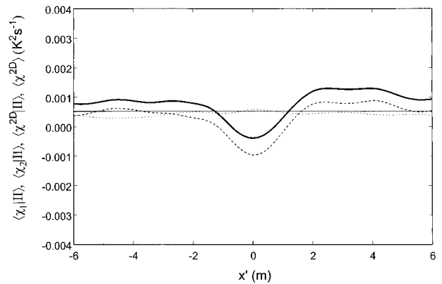
FIG. 12. Conditionally averaged surrogates of the SGS dissipation of temperature variance, under condition II ( \partial\theta/\partial t > \sigma_{\text{ab}(\text{oi})} ), for measurement period U (unstable surface layer). Streamwise component \langle \chi_1 | II \rangle (dashed line), spanwise component \langle \chi_2 | II \rangle (dotted line), and 2D surrogate \langle \chi^{2D} | II \rangle (thick solid line). The light solid line corresponds to the overall mean 2D surrogate of the SGS dissipation \langle \chi^{2D} \rangle .
