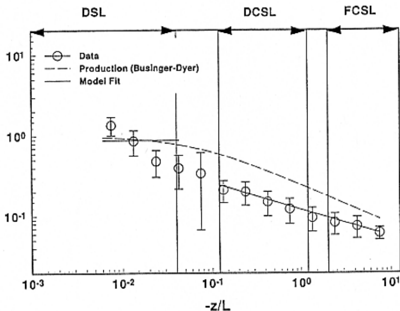
Figure 4. Data from Figure 2c placed in logarithmically spaced bins. The average of the \Phi_{\epsilon_\theta} data in each bin is represented with an open circle, and the standard deviations are marked with vertical bars. The Businger-Dyer production model is shown as a dashed line and the derived dissipation scaling (20) is plotted with the solid line. The near-neutral outlier of figure 2c has been omitted.
