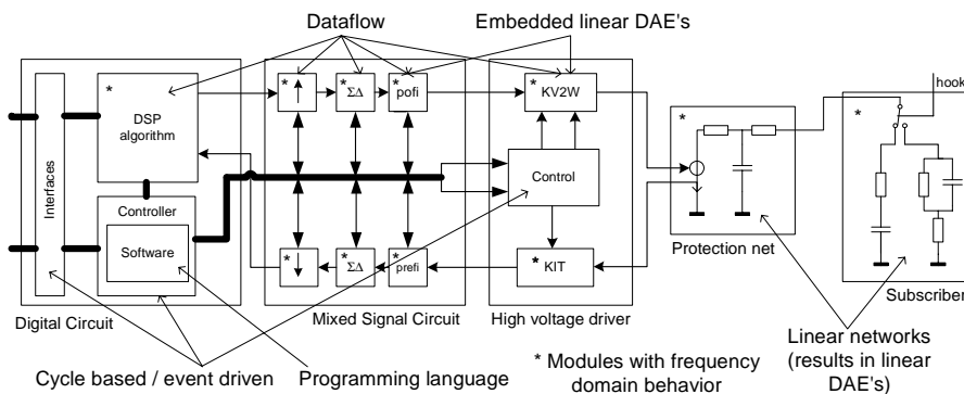
Figure 1. Simplified block diagram of a subscriber line interface and codec filter.
