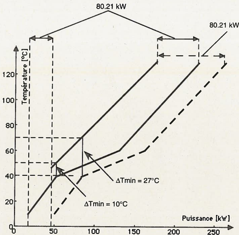
Figure 9: Cas limite de composites relatives aux flux de la table 2.
