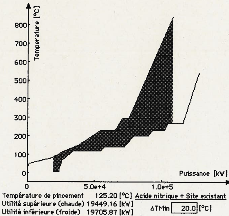
Figure 12c: Composites acide nitrique + site existant
