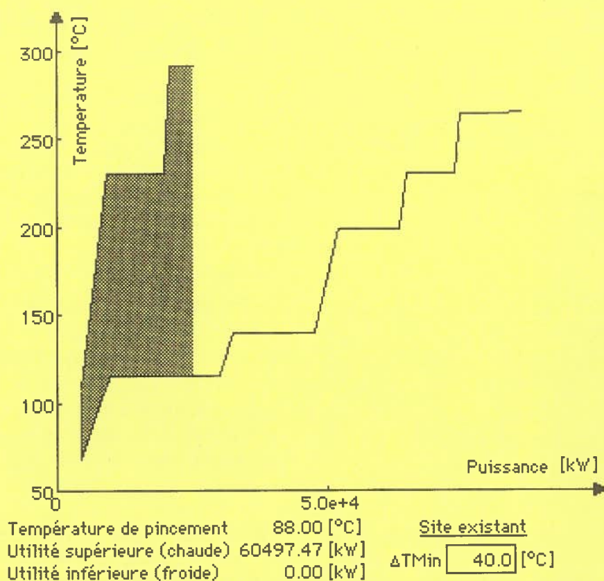
Figure 4b: Composites du site existant.
