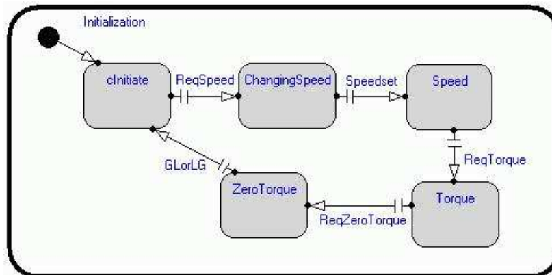
Figure 12: Statechart Diagram Engine Component.
