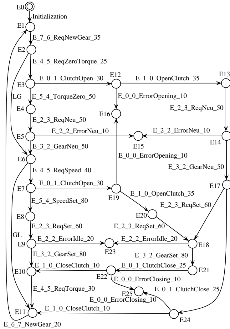
Figure 8: Finite State Model of Gear Controller.
